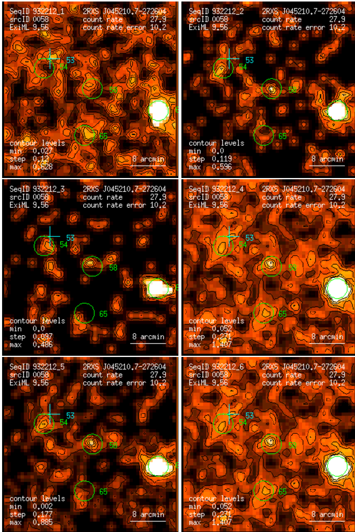
Figure 58: RASS 932212: detection 0058: band rate images, Gaussian filter: (1) PSPC channels 11 – 41, (2) 52 – 90, (3) 91 – 201, (4) 11 – 235, (5) 52 – 201, (6) 11 – 201. Broad band rates in counts/ks. Band rate contour levels in counts/ks/arcmin 2 .
