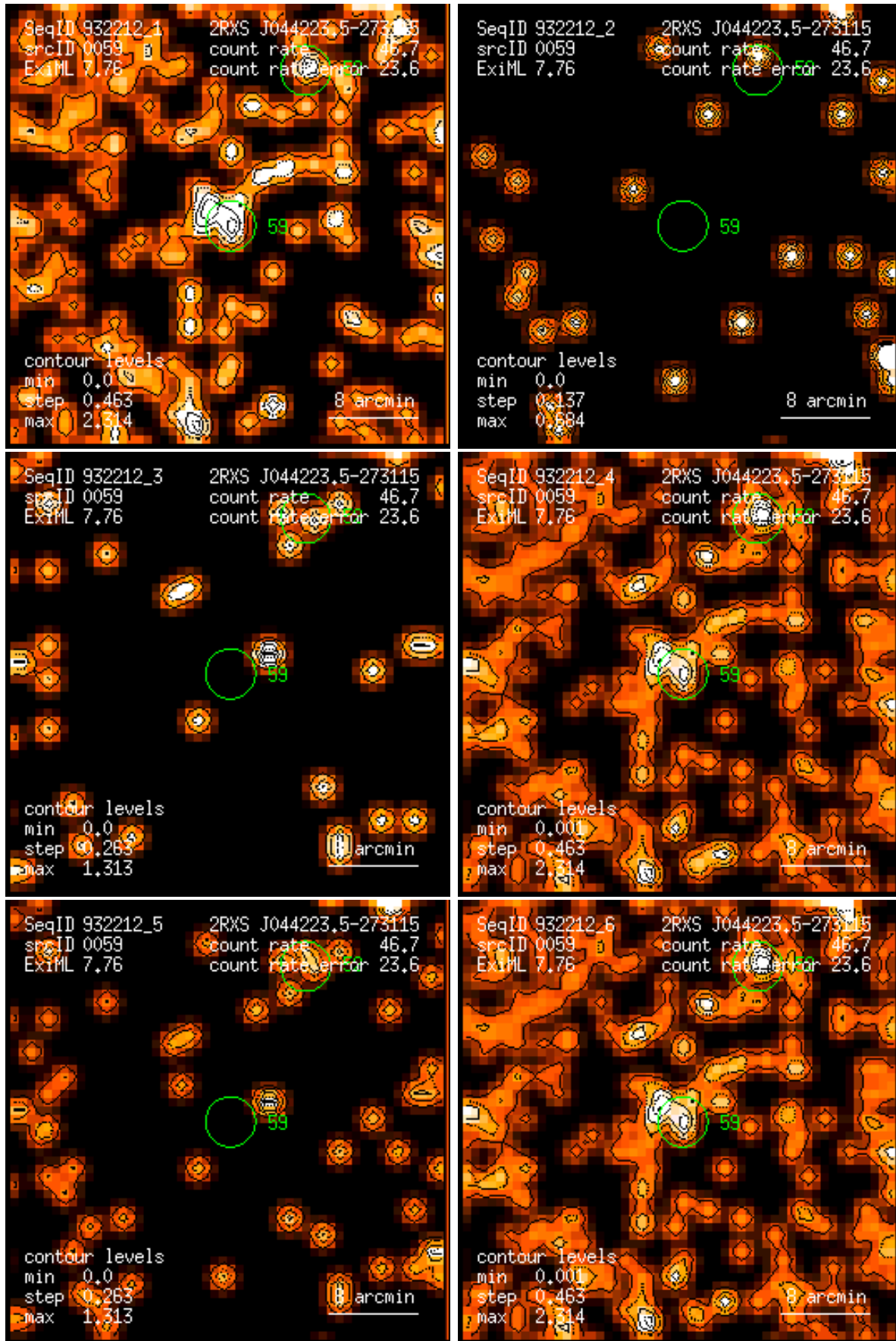
Figure 59: RASS 932212: detection 0059: band rate images, Gaussian filter: (1) PSPC channels 11 – 41, (2) 52 – 90, (3) 91 – 201, (4) 11 – 235, (5) 52 – 201, (6) 11 – 201. Broad band rates in counts/ks. Band rate contour levels in counts/ks/arcmin 2 .
