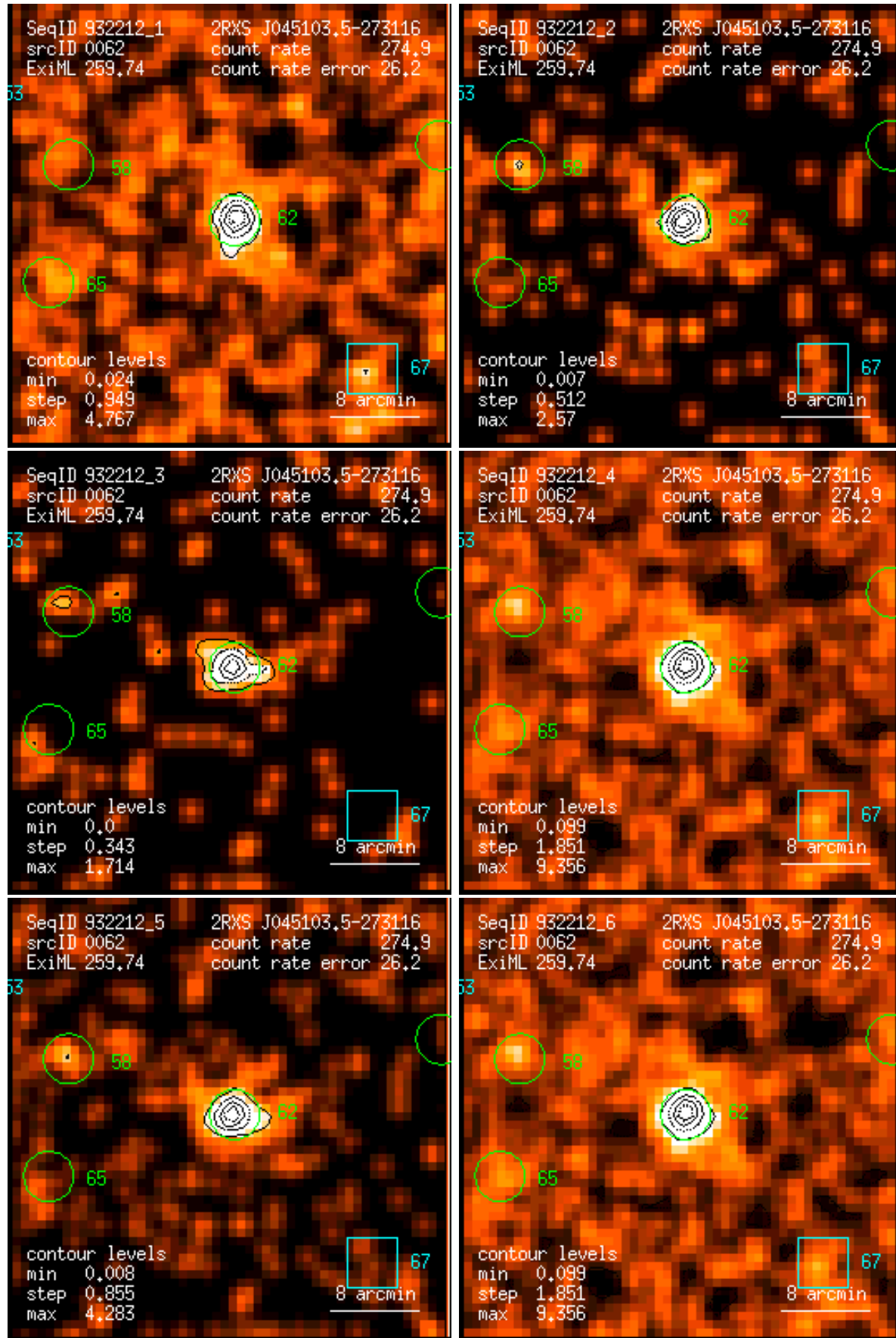
Figure 62: RASS 932212: detection 0062: band rate images, Gaussian filter: (1) PSPC channels 11 – 41, (2) 52 – 90, (3) 91 – 201, (4) 11 – 235, (5) 52 – 201, (6) 11 – 201. Broad band rates in counts/ks. Band rate contour levels in counts/ks/arcmin 2 .
