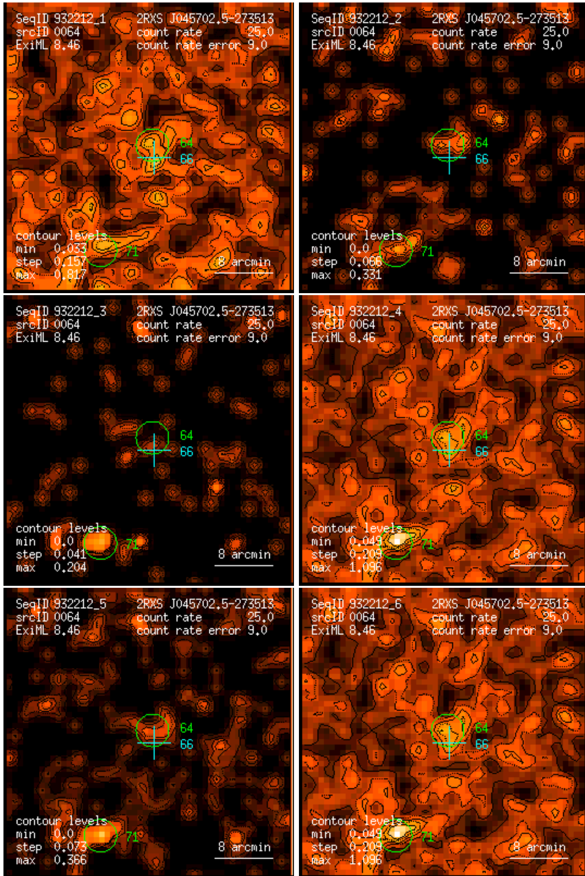
Figure 64: RASS 932212: detection 0064: band rate images, Gaussian filter: (1) PSPC channels 11 – 41, (2) 52 – 90, (3) 91 – 201, (4) 11 – 235, (5) 52 – 201, (6) 11 – 201. Broad band rates in counts/ks. Band rate contour levels in counts/ks/arcmin 2 .
