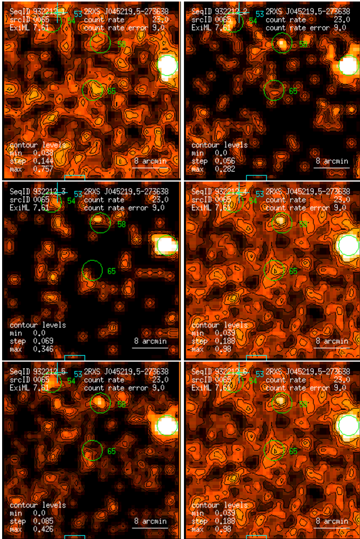
Figure 65: RASS 932212: detection 0065: band rate images, Gaussian filter: (1) PSPC channels 11 – 41, (2) 52 – 90, (3) 91 – 201, (4) 11 – 235, (5) 52 – 201, (6) 11 – 201. Broad band rates in counts/ks. Band rate contour levels in counts/ks/arcmin 2 .
