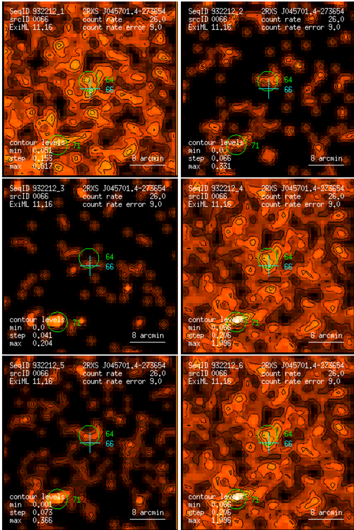
Figure 66: RASS 932212: detection 0066: band rate images, Gaussian filter: (1) PSPC channels 11 – 41, (2) 52 – 90, (3) 91 – 201, (4) 11 – 235, (5) 52 – 201, (6) 11 – 201. Broad band rates in counts/ks. Band rate contour levels in counts/ks/arcmin 2 .
