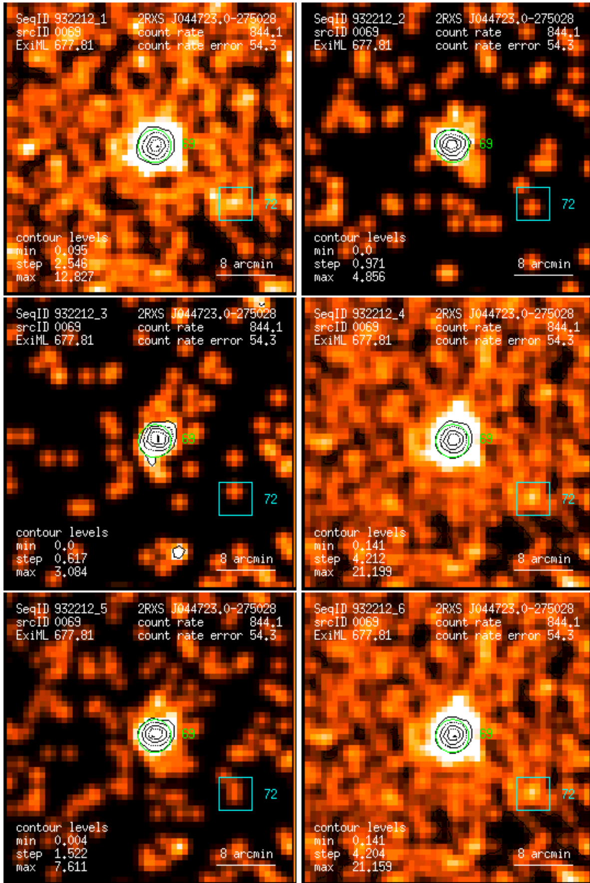
Figure 69: RASS 932212: detection 0069: band rate images, Gaussian filter: (1) PSPC channels 11 – 41, (2) 52 – 90, (3) 91 – 201, (4) 11 – 235, (5) 52 – 201, (6) 11 – 201. Broad band rates in counts/ks. Band rate contour levels in counts/ks/arcmin 2 .
