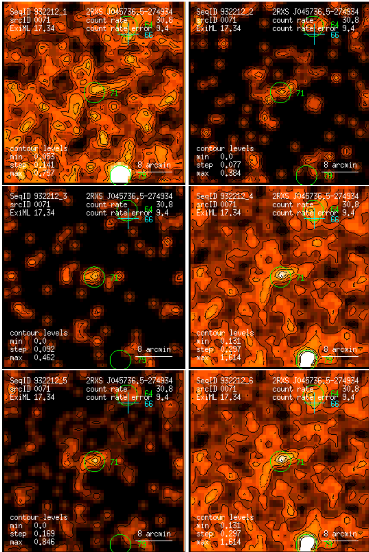
Figure 71: RASS 932212: detection 0071: band rate images, Gaussian filter: (1) PSPC channels 11 – 41, (2) 52 – 90, (3) 91 – 201, (4) 11 – 235, (5) 52 – 201, (6) 11 – 201. Broad band rates in counts/ks. Band rate contour levels in counts/ks/arcmin 2 .
