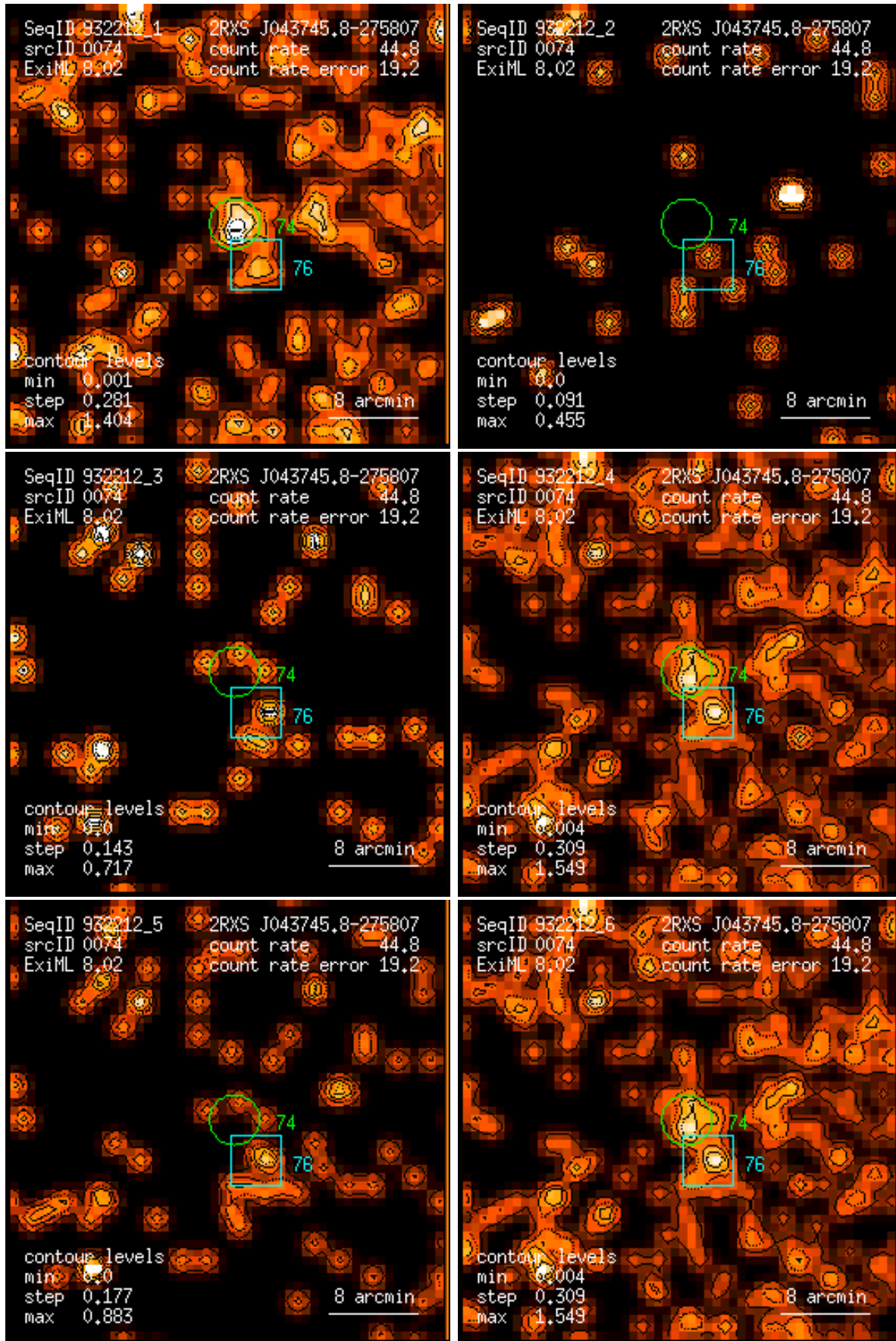
Figure 74: RASS 932212: detection 0074: band rate images, Gaussian filter: (1) PSPC channels 11 – 41, (2) 52 – 90, (3) 91 – 201, (4) 11 – 235, (5) 52 – 201, (6) 11 – 201. Broad band rates in counts/ks. Band rate contour levels in counts/ks/arcmin 2 .
