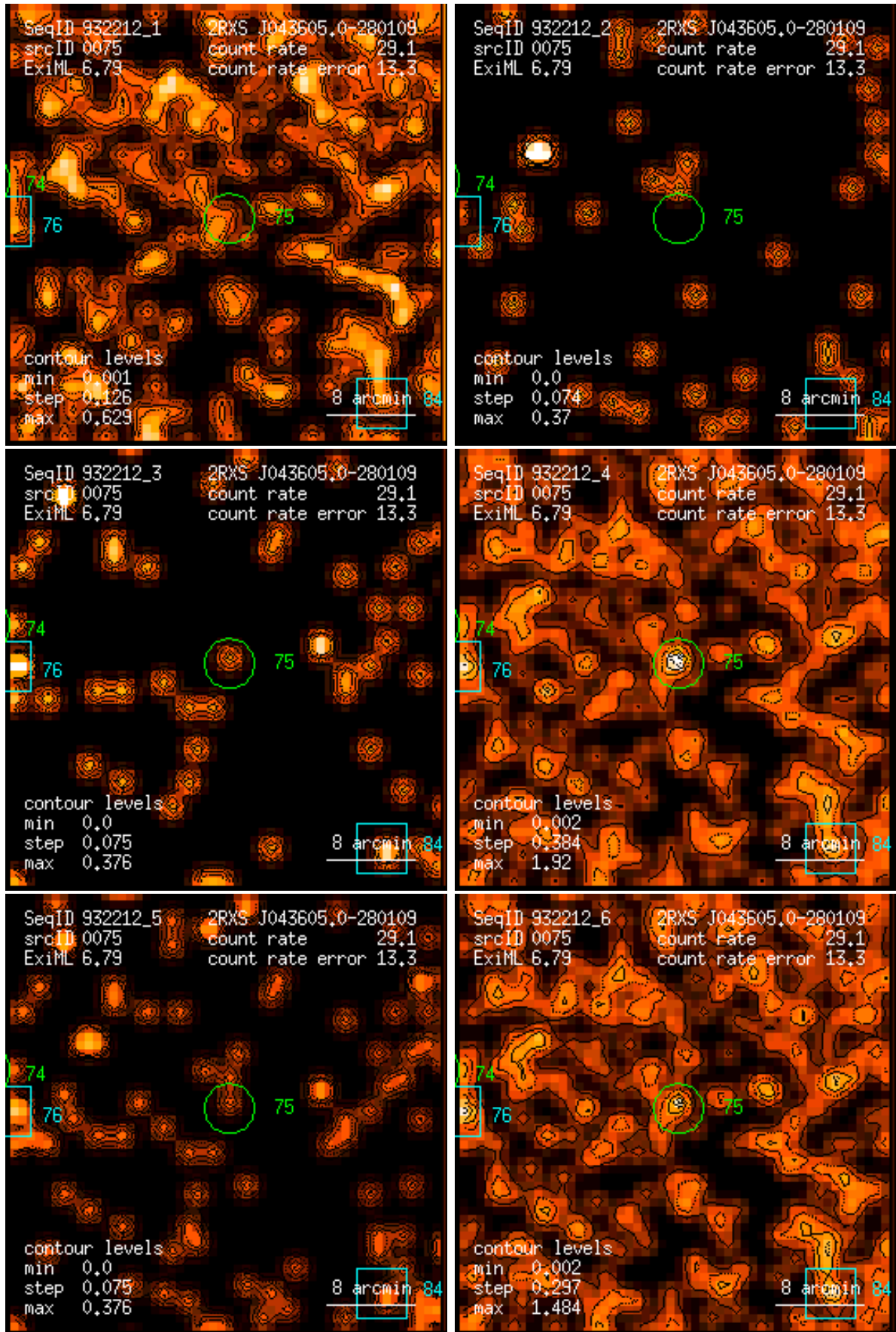
Figure 75: RASS 932212: detection 0075: band rate images, Gaussian filter: (1) PSPC channels 11 – 41, (2) 52 – 90, (3) 91 – 201, (4) 11 – 235, (5) 52 – 201, (6) 11 – 201. Broad band rates in counts/ks. Band rate contour levels in counts/ks/arcmin 2 .
