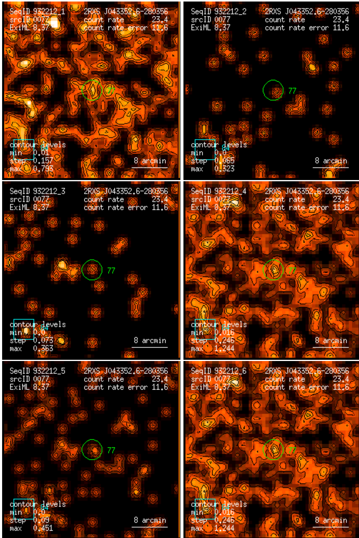
Figure 77: RASS 932212: detection 0077: band rate images, Gaussian filter: (1) PSPC channels 11 – 41, (2) 52 – 90, (3) 91 – 201, (4) 11 – 235, (5) 52 – 201, (6) 11 – 201. Broad band rates in counts/ks. Band rate contour levels in counts/ks/arcmin 2 .
