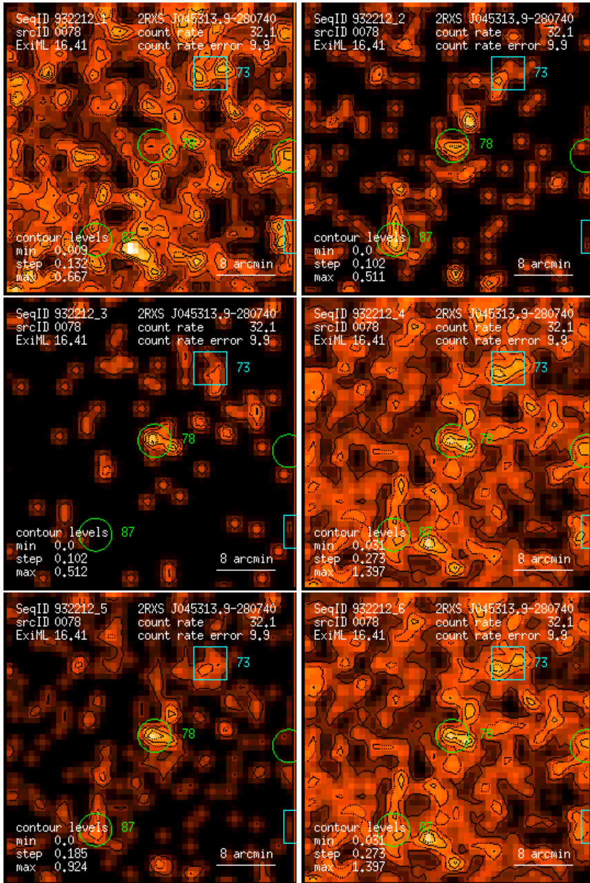
Figure 78: RASS 932212: detection 0078: band rate images, Gaussian filter: (1) PSPC channels 11 – 41, (2) 52 – 90, (3) 91 – 201, (4) 11 – 235, (5) 52 – 201, (6) 11 – 201. Broad band rates in counts/ks. Band rate contour levels in counts/ks/arcmin 2 .
