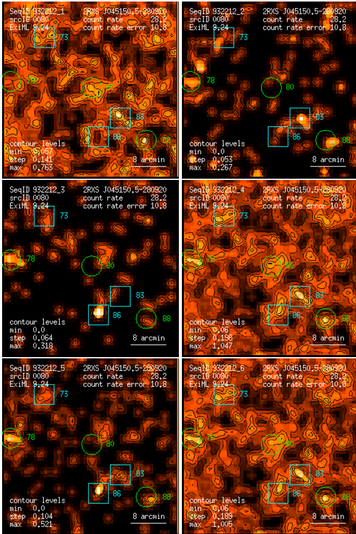
Figure 80: RASS 932212: detection 0080: band rate images, Gaussian filter: (1) PSPC channels 11 – 41, (2) 52 – 90, (3) 91 – 201, (4) 11 – 235, (5) 52 – 201, (6) 11 – 201. Broad band rates in counts/ks. Band rate contour levels in counts/ks/arcmin 2 .
