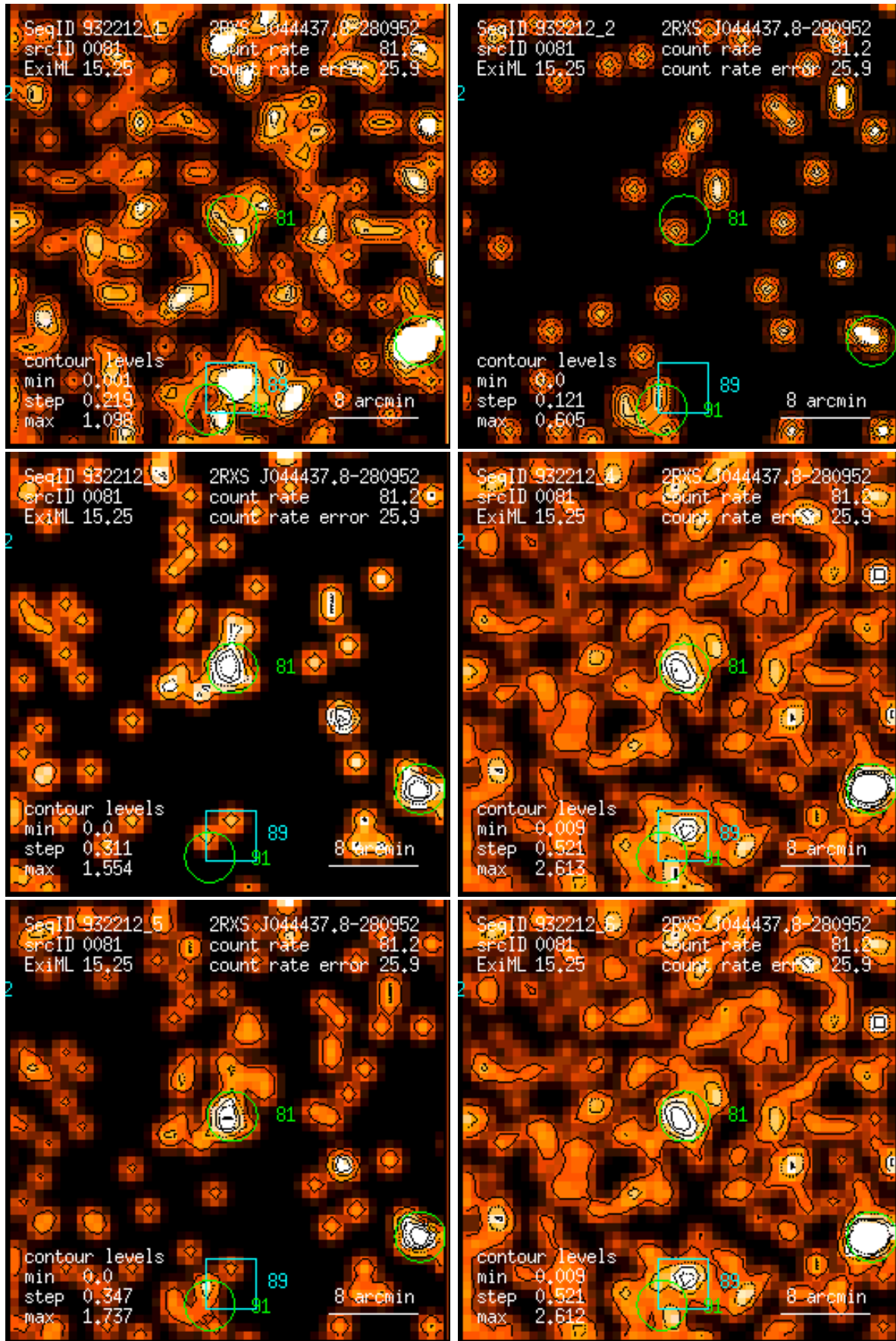
Figure 81: RASS 932212: detection 0081: band rate images, Gaussian filter: (1) PSPC channels 11 – 41, (2) 52 – 90, (3) 91 – 201, (4) 11 – 235, (5) 52 – 201, (6) 11 – 201. Broad band rates in counts/ks. Band rate contour levels in counts/ks/arcmin 2 .
