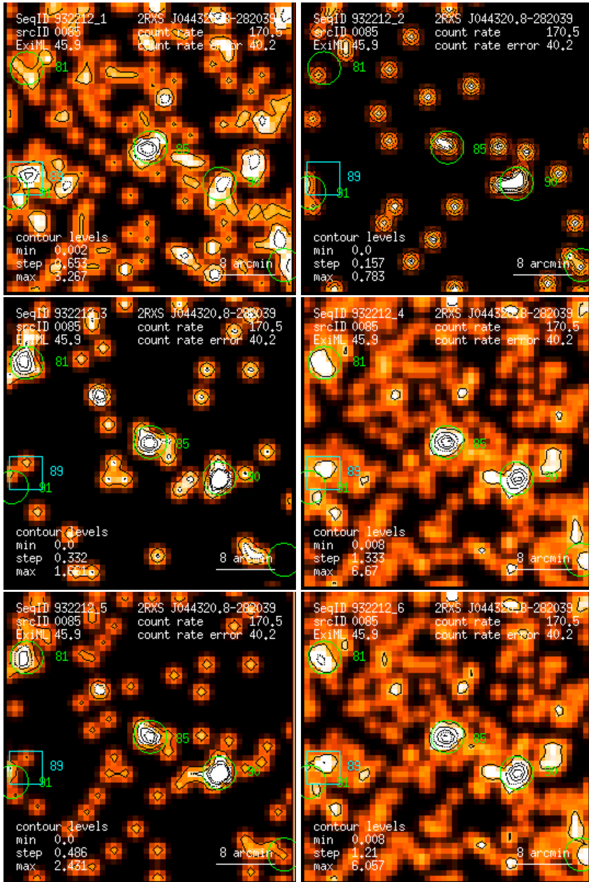
Figure 85: RASS 932212: detection 0085: band rate images, Gaussian filter: (1) PSPC channels 11 – 41, (2) 52 – 90, (3) 91 – 201, (4) 11 – 235, (5) 52 – 201, (6) 11 – 201. Broad band rates in counts/ks. Band rate contour levels in counts/ks/arcmin 2 .
