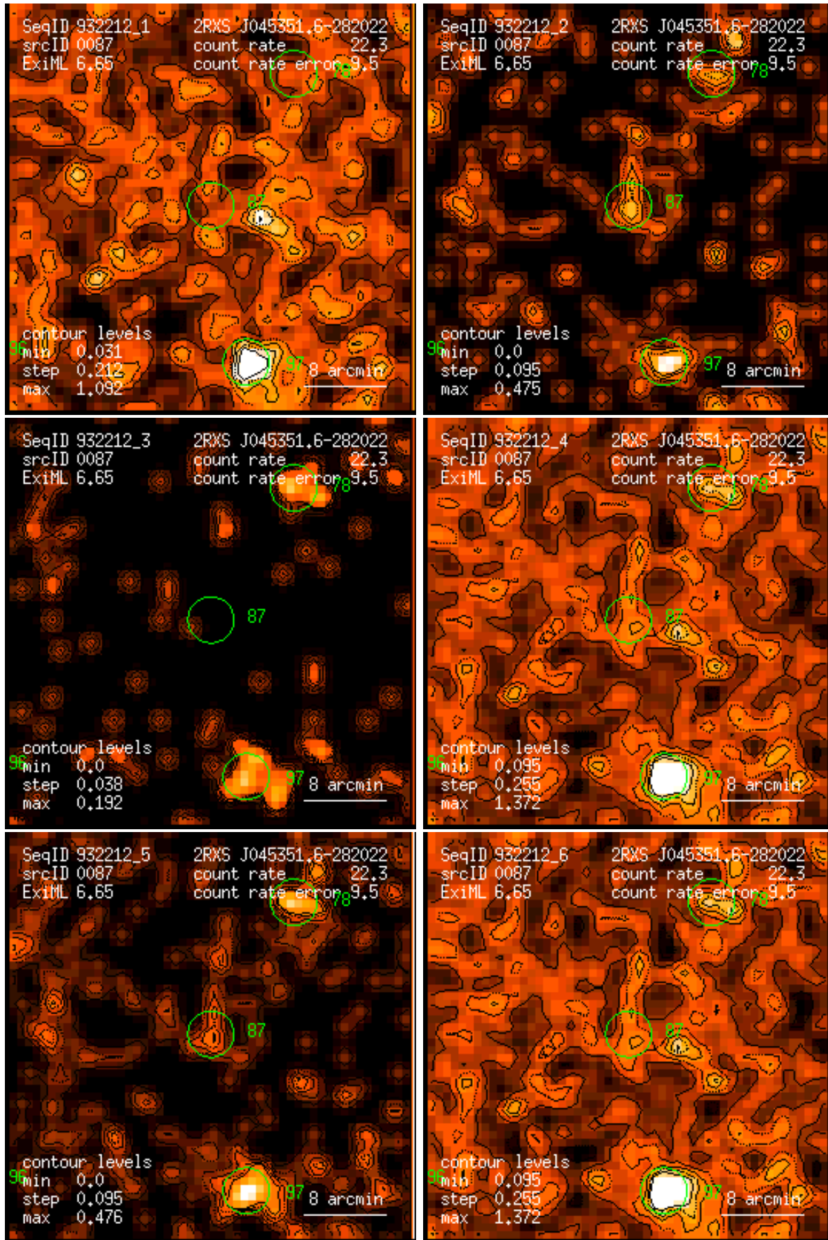
Figure 87: RASS 932212: detection 0087: band rate images, Gaussian filter: (1) PSPC channels 11 – 41, (2) 52 – 90, (3) 91 – 201, (4) 11 – 235, (5) 52 – 201, (6) 11 – 201. Broad band rates in counts/ks. Band rate contour levels in counts/ks/arcmin 2 .
