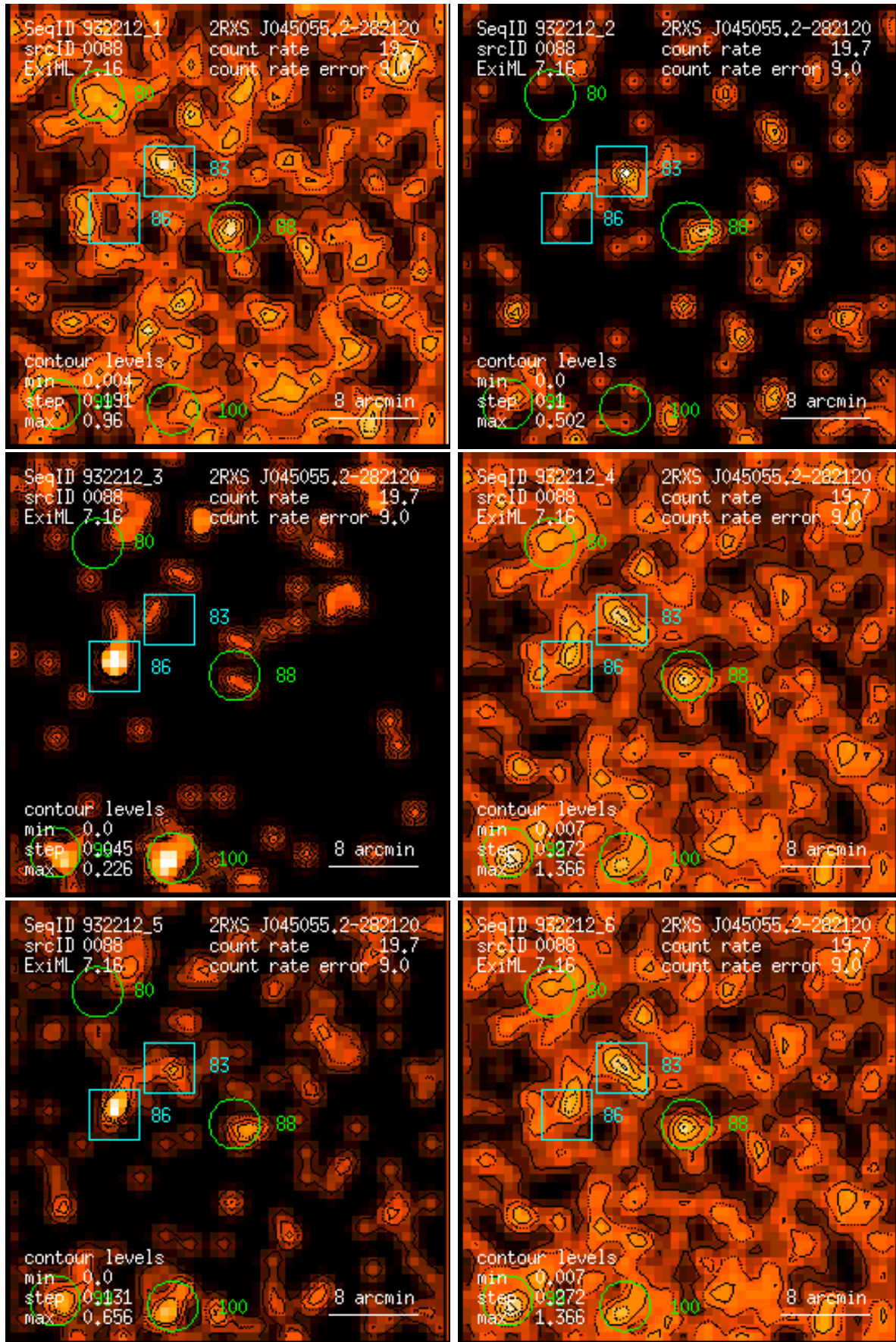
Figure 88: RASS 932212: detection 0088: band rate images, Gaussian filter: (1) PSPC channels 11 – 41, (2) 52 – 90, (3) 91 – 201, (4) 11 – 235, (5) 52 – 201, (6) 11 – 201. Broad band rates in counts/ks. Band rate contour levels in counts/ks/arcmin 2 .
