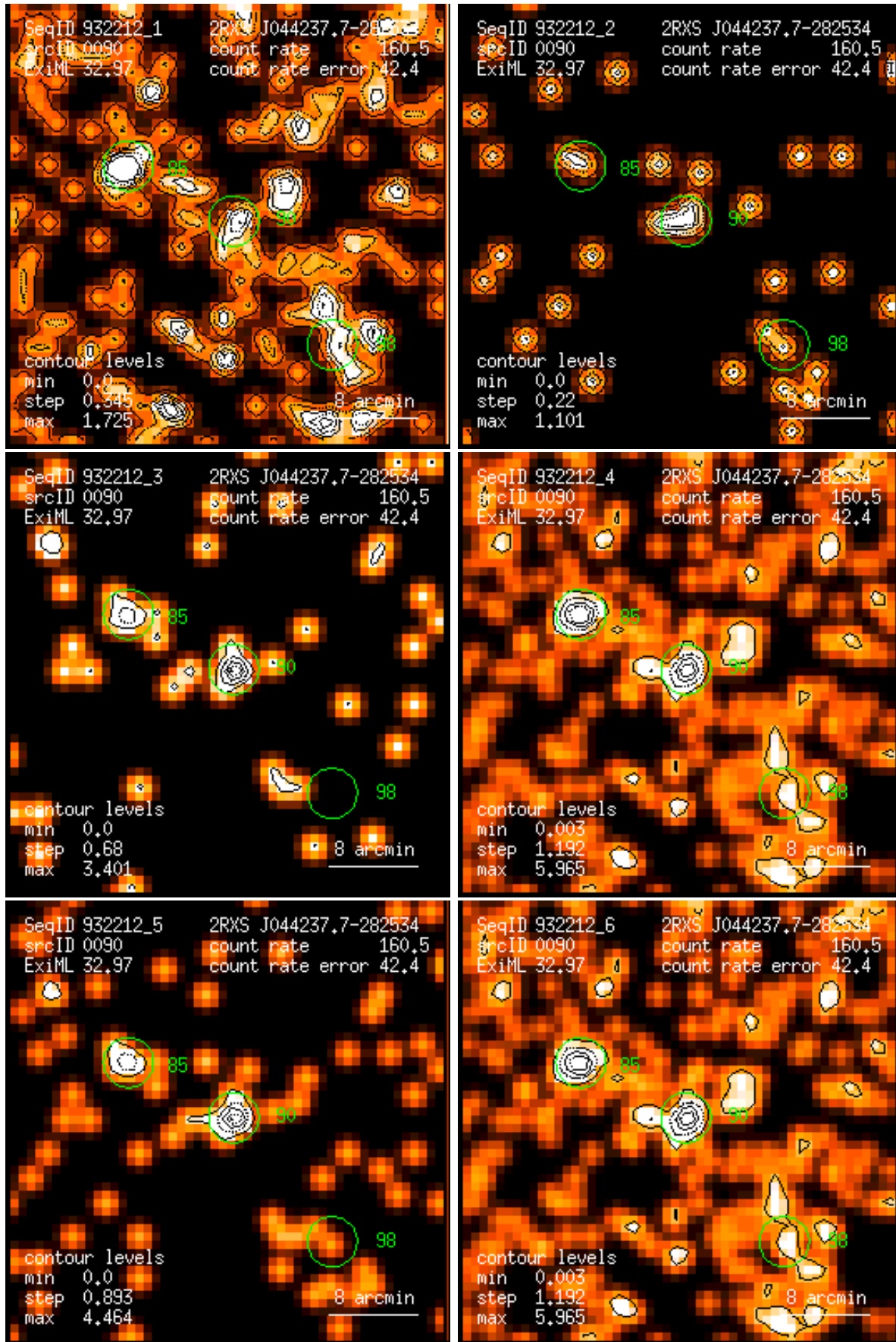
Figure 90: RASS 932212: detection 0090: band rate images, Gaussian filter: (1) PSPC channels 11 – 41, (2) 52 – 90, (3) 91 – 201, (4) 11 – 235, (5) 52 – 201, (6) 11 – 201. Broad band rates in counts/ks. Band rate contour levels in counts/ks/arcmin 2 .
