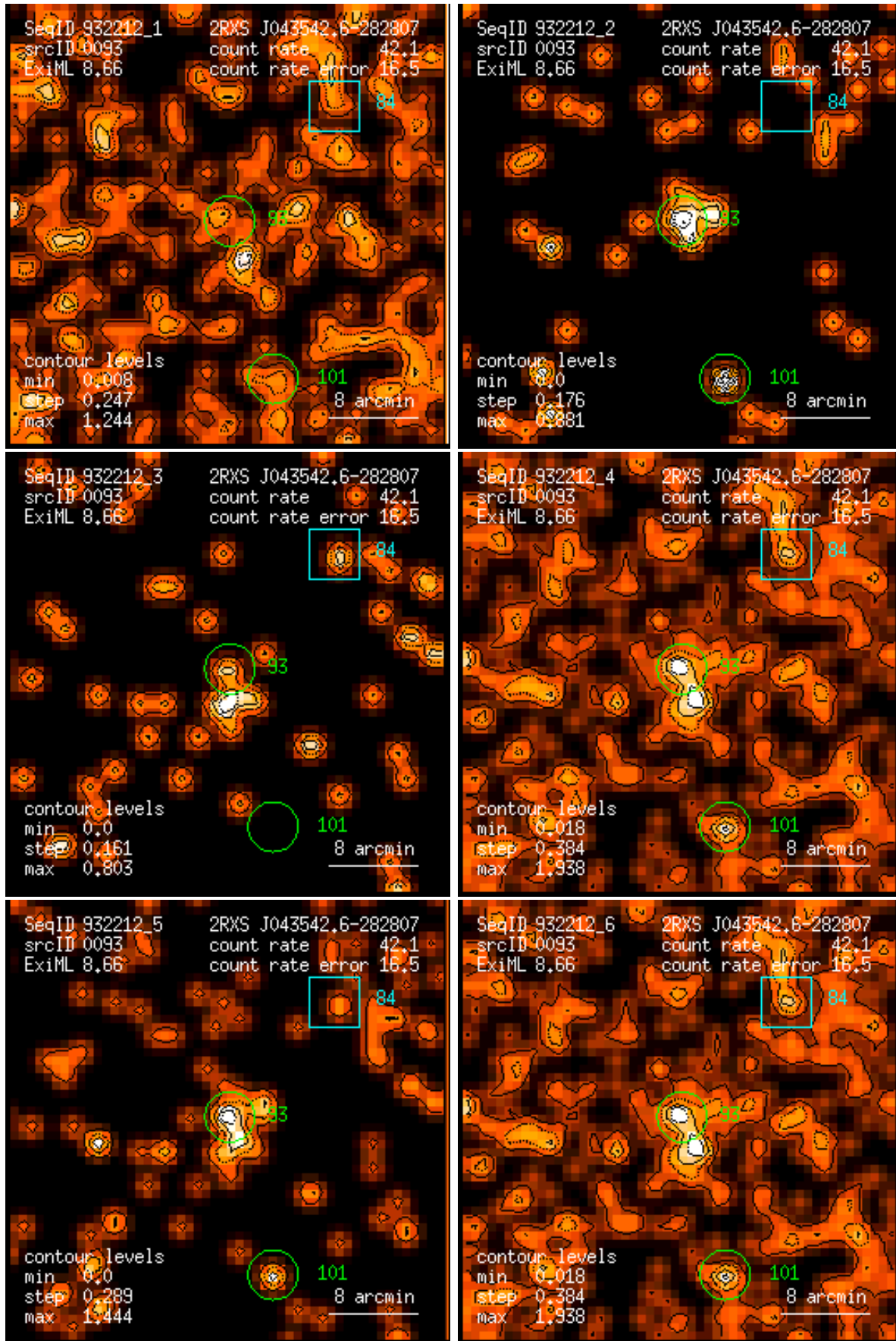
Figure 93: RASS 932212: detection 0093: band rate images, Gaussian filter: (1) PSPC channels 11 – 41, (2) 52 – 90, (3) 91 – 201, (4) 11 – 235, (5) 52 – 201, (6) 11 – 201. Broad band rates in counts/ks. Band rate contour levels in counts/ks/arcmin 2 .
