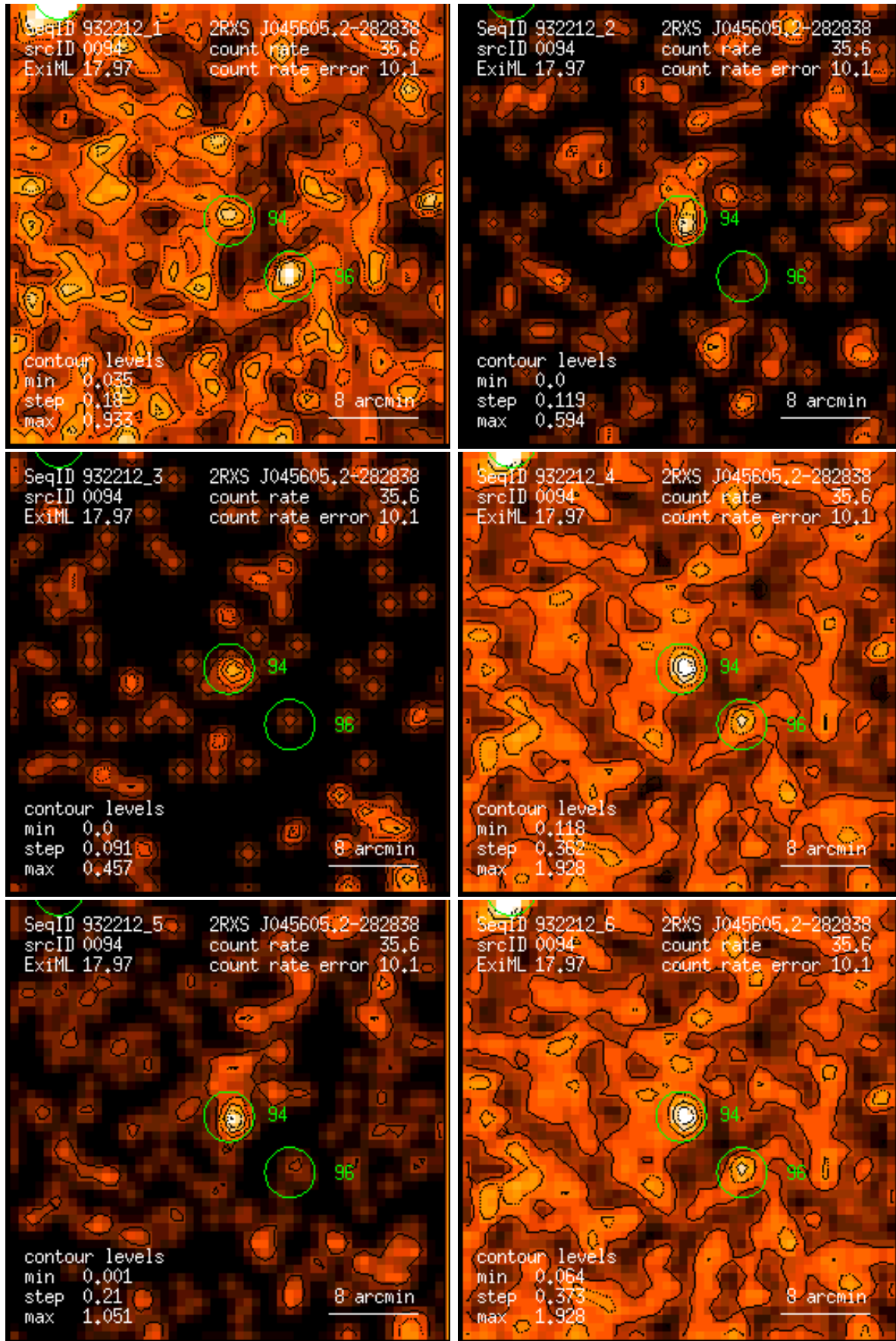
Figure 94: RASS 932212: detection 0094: band rate images, Gaussian filter: (1) PSPC channels 11 – 41, (2) 52 – 90, (3) 91 – 201, (4) 11 – 235, (5) 52 – 201, (6) 11 – 201. Broad band rates in counts/ks. Band rate contour levels in counts/ks/arcmin 2 .
