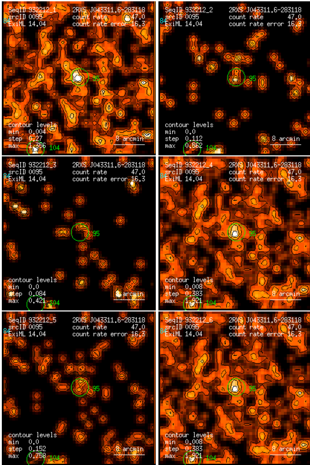
Figure 95: RASS 932212: detection 0095: band rate images, Gaussian filter: (1) PSPC channels 11 – 41, (2) 52 – 90, (3) 91 – 201, (4) 11 – 235, (5) 52 – 201, (6) 11 – 201. Broad band rates in counts/ks. Band rate contour levels in counts/ks/arcmin 2 .
