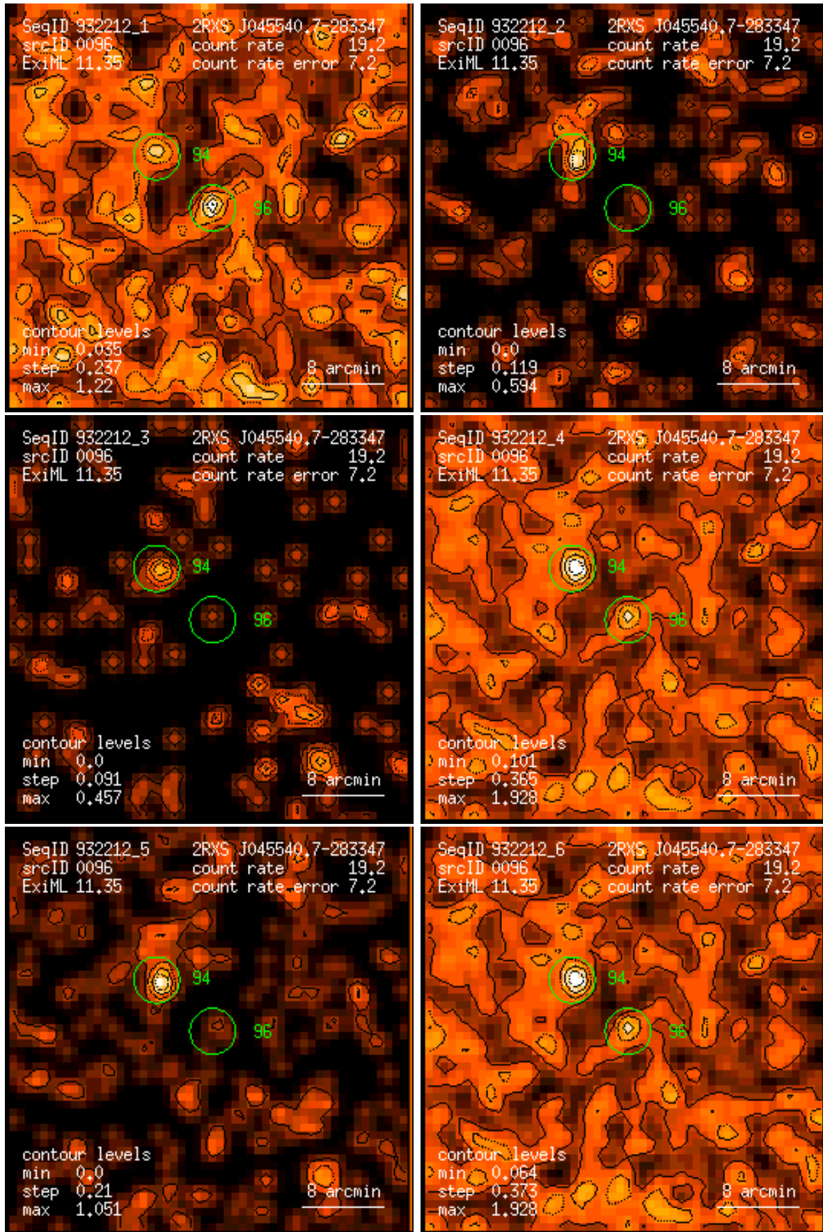
Figure 96: RASS 932212: detection 0096: band rate images, Gaussian filter: (1) PSPC channels 11 – 41, (2) 52 – 90, (3) 91 – 201, (4) 11 – 235, (5) 52 – 201, (6) 11 – 201. Broad band rates in counts/ks. Band rate contour levels in counts/ks/arcmin 2 .
