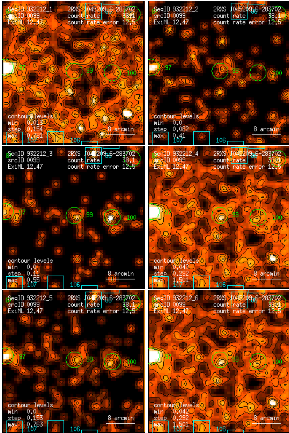
Figure 99: RASS 932212: detection 0099: band rate images, Gaussian filter: (1) PSPC channels 11 – 41, (2) 52 – 90, (3) 91 – 201, (4) 11 – 235, (5) 52 – 201, (6) 11 – 201. Broad band rates in counts/ks. Band rate contour levels in counts/ks/arcmin 2 .
