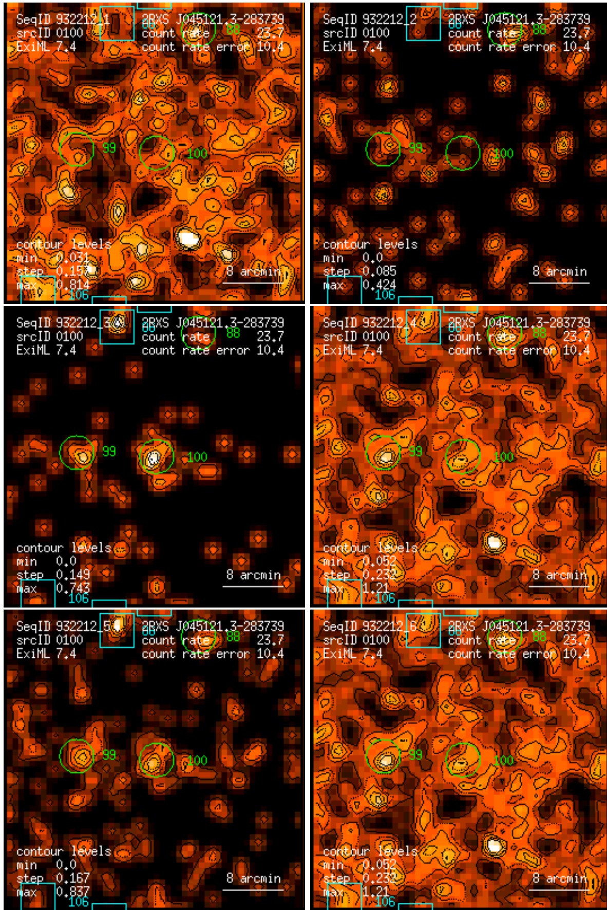
Figure 100: RASS 932212: detection 0100: band rate images, Gaussian filter: (1) PSPC channels 11 – 41, (2) 52 – 90, (3) 91 – 201, (4) 11 – 235, (5) 52 – 201, (6) 11 – 201. Broad band rates in counts/ks. Band rate contour levels in counts/ks/arcmin 2 .
