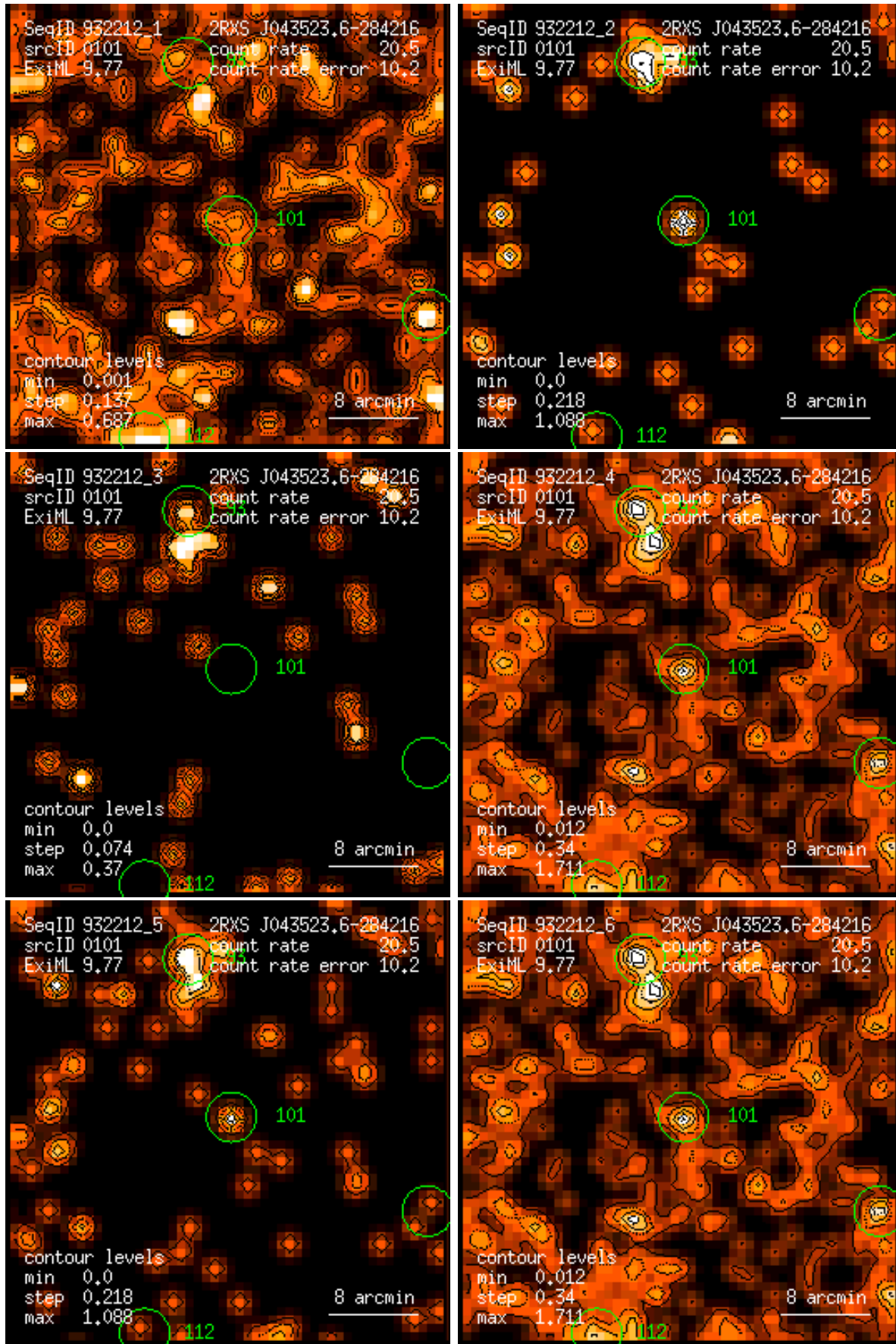
Figure 101: RASS 932212: detection 0101: band rate images, Gaussian filter: (1) PSPC channels 11 – 41, (2) 52 – 90, (3) 91 – 201, (4) 11 – 235, (5) 52 – 201, (6) 11 – 201. Broad band rates in counts/ks. Band rate contour levels in counts/ks/arcmin 2 .
