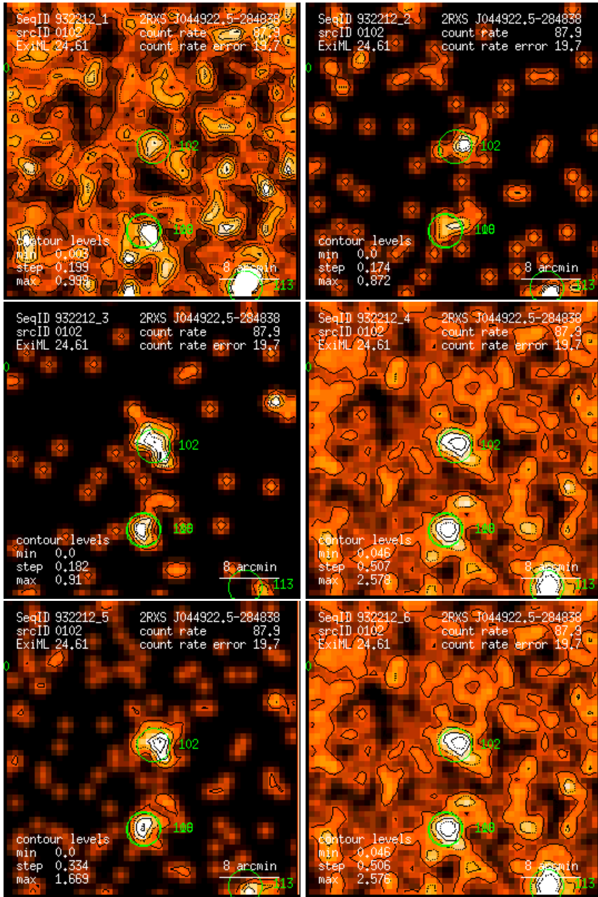
Figure 102: RASS 932212: detection 0102: band rate images, Gaussian filter: (1) PSPC channels 11 – 41, (2) 52 – 90, (3) 91 – 201, (4) 11 – 235, (5) 52 – 201, (6) 11 – 201. Broad band rates in counts/ks. Band rate contour levels in counts/ks/arcmin 2 .
