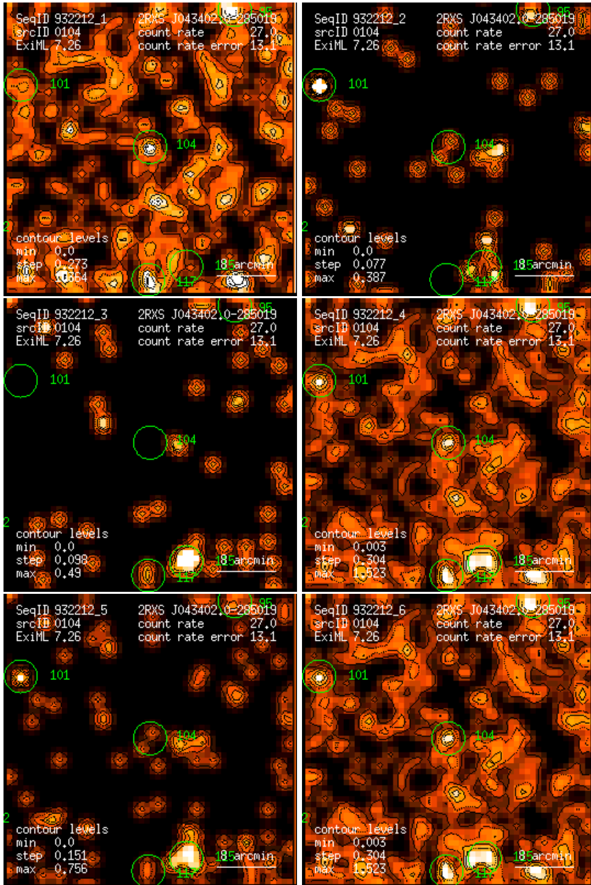
Figure 104: RASS 932212: detection 0104: band rate images, Gaussian filter: (1) PSPC channels 11 – 41, (2) 52 – 90, (3) 91 – 201, (4) 11 – 235, (5) 52 – 201, (6) 11 – 201. Broad band rates in counts/ks. Band rate contour levels in counts/ks/arcmin 2 .
