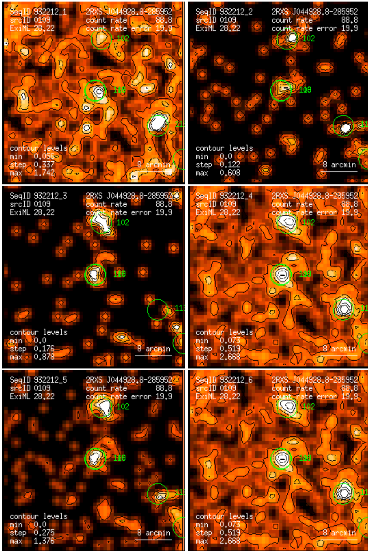
Figure 109: RASS 932212: detection 0109: band rate images, Gaussian filter: (1) PSPC channels 11 – 41, (2) 52 – 90, (3) 91 – 201, (4) 11 – 235, (5) 52 – 201, (6) 11 – 201. Broad band rates in counts/ks. Band rate contour levels in counts/ks/arcmin 2 .
