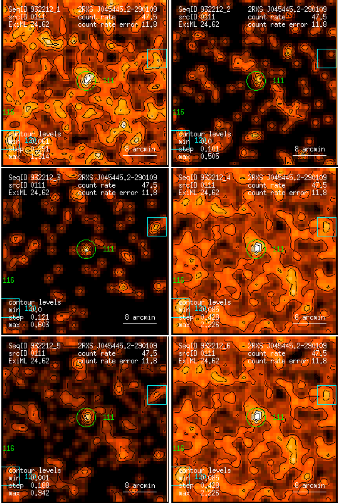
Figure 111: RASS 932212: detection 0111: band rate images, Gaussian filter: (1) PSPC channels 11 – 41, (2) 52 – 90, (3) 91 – 201, (4) 11 – 235, (5) 52 – 201, (6) 11 – 201. Broad band rates in counts/ks. Band rate contour levels in counts/ks/arcmin 2 .
