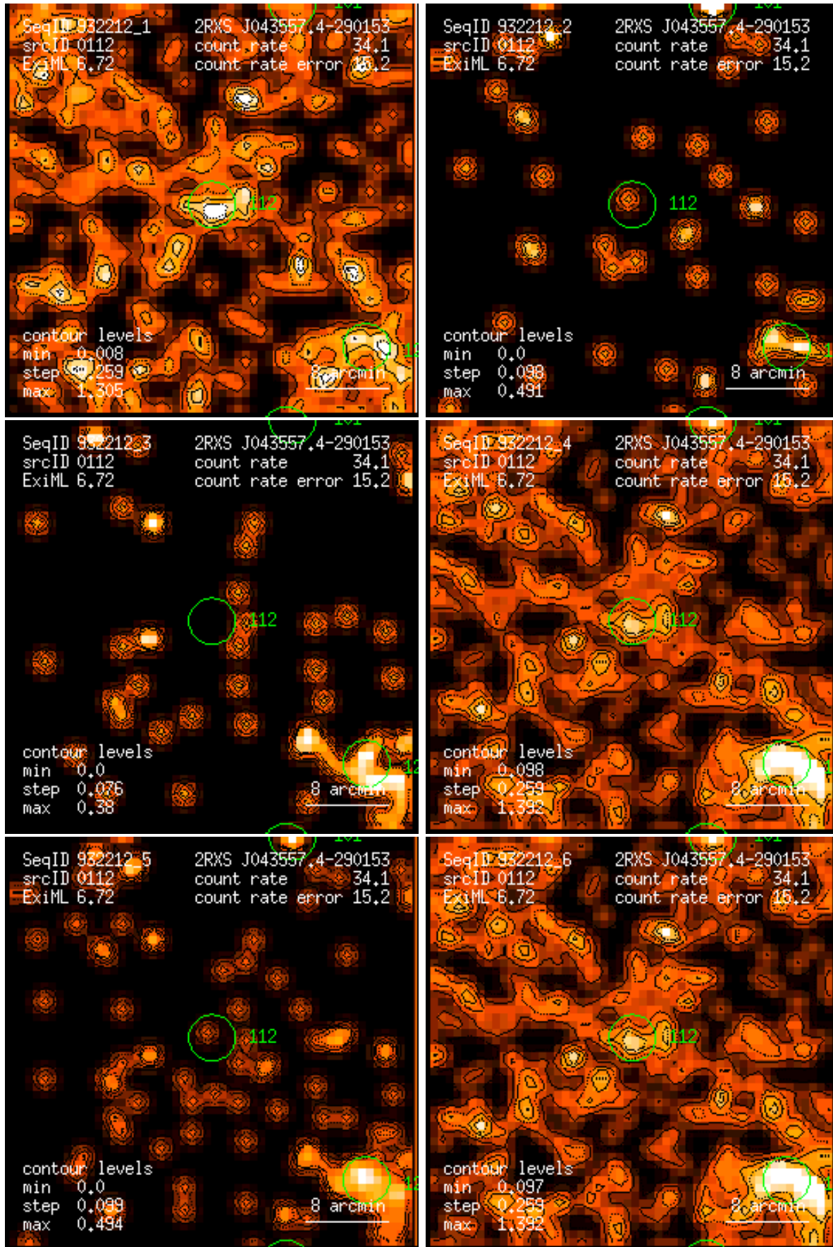
Figure 112: RASS 932212: detection 0112: band rate images, Gaussian filter: (1) PSPC channels 11 – 41, (2) 52 – 90, (3) 91 – 201, (4) 11 – 235, (5) 52 – 201, (6) 11 – 201. Broad band rates in counts/ks. Band rate contour levels in counts/ks/arcmin 2 .
