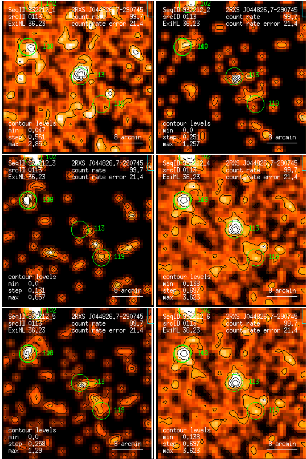
Figure 113: RASS 932212: detection 0113: band rate images, Gaussian filter: (1) PSPC channels 11 – 41, (2) 52 – 90, (3) 91 – 201, (4) 11 – 235, (5) 52 – 201, (6) 11 – 201. Broad band rates in counts/ks. Band rate contour levels in counts/ks/arcmin 2 .
