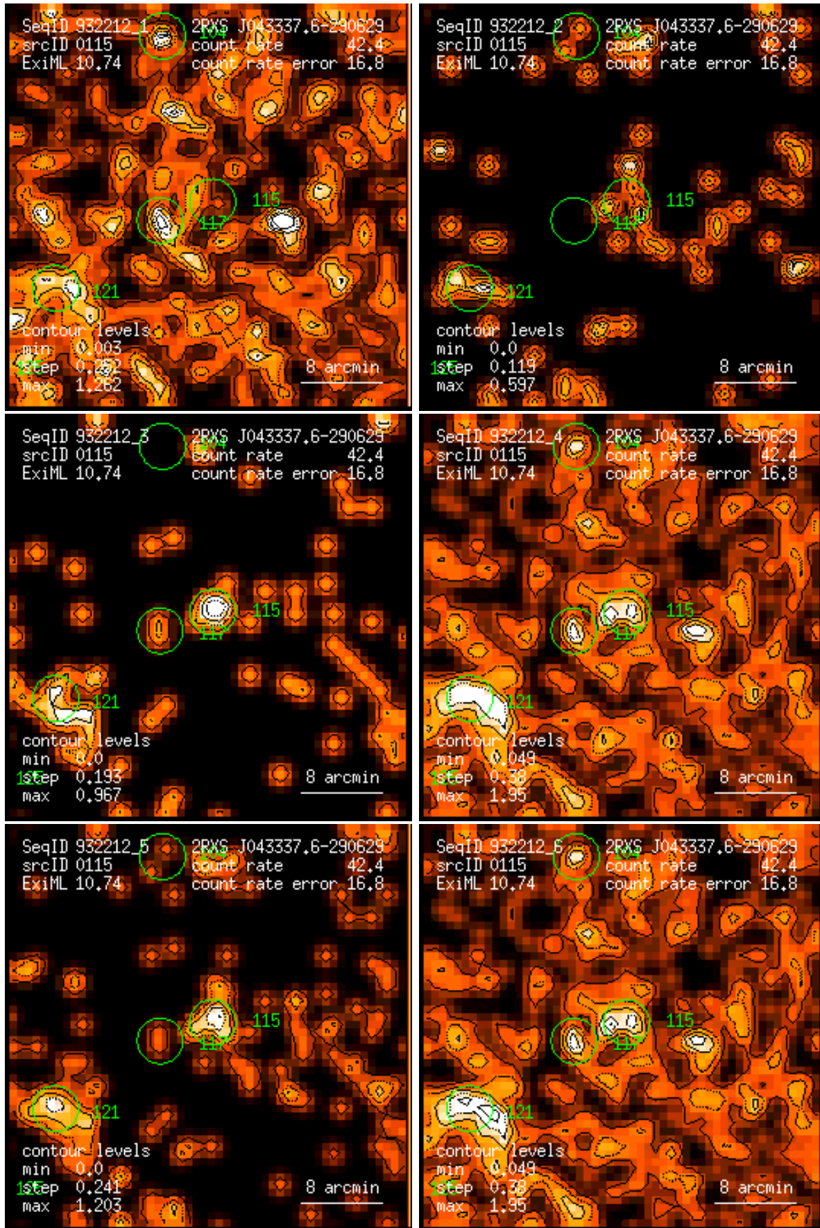
Figure 115: RASS 932212: detection 0115: band rate images, Gaussian filter: (1) PSPC channels 11 – 41, (2) 52 – 90, (3) 91 – 201, (4) 11 – 235, (5) 52 – 201, (6) 11 – 201. Broad band rates in counts/ks. Band rate contour levels in counts/ks/arcmin 2 .
