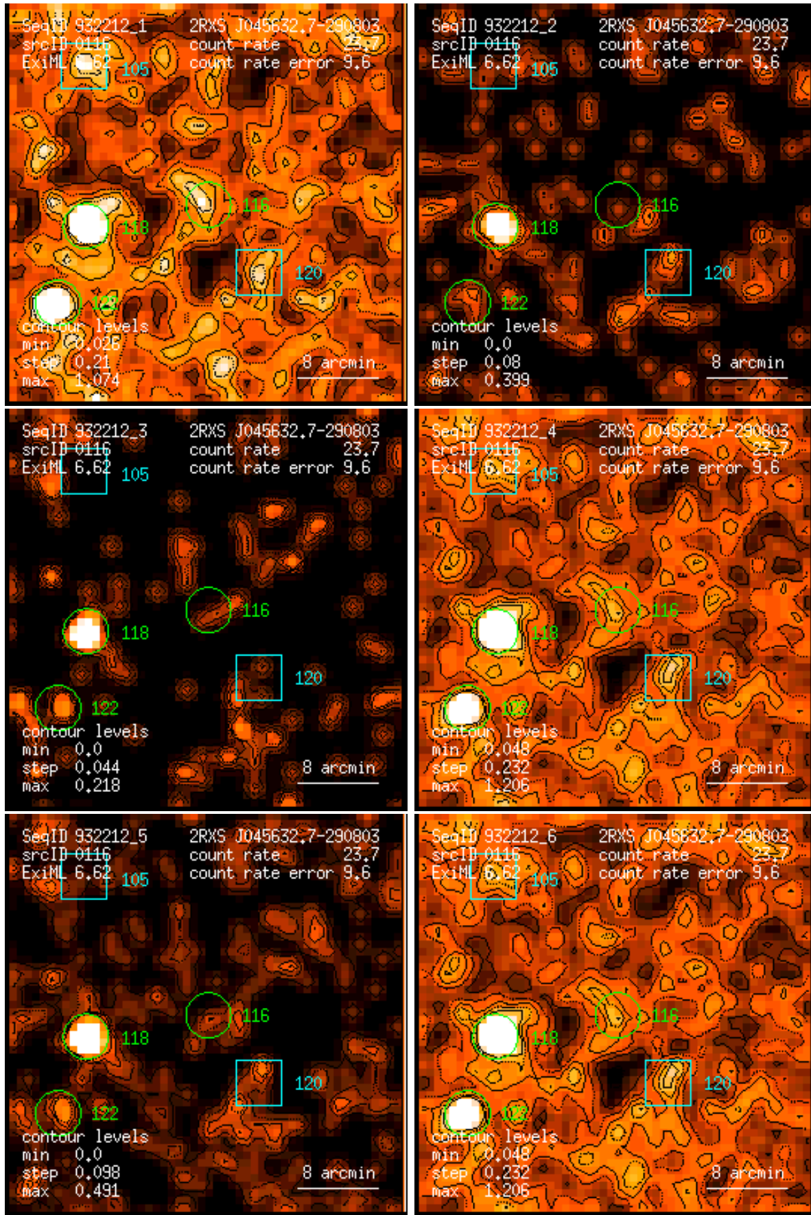
Figure 116: RASS 932212: detection 0116: band rate images, Gaussian filter: (1) PSPC channels 11 – 41, (2) 52 – 90, (3) 91 – 201, (4) 11 – 235, (5) 52 – 201, (6) 11 – 201. Broad band rates in counts/ks. Band rate contour levels in counts/ks/arcmin 2 .
