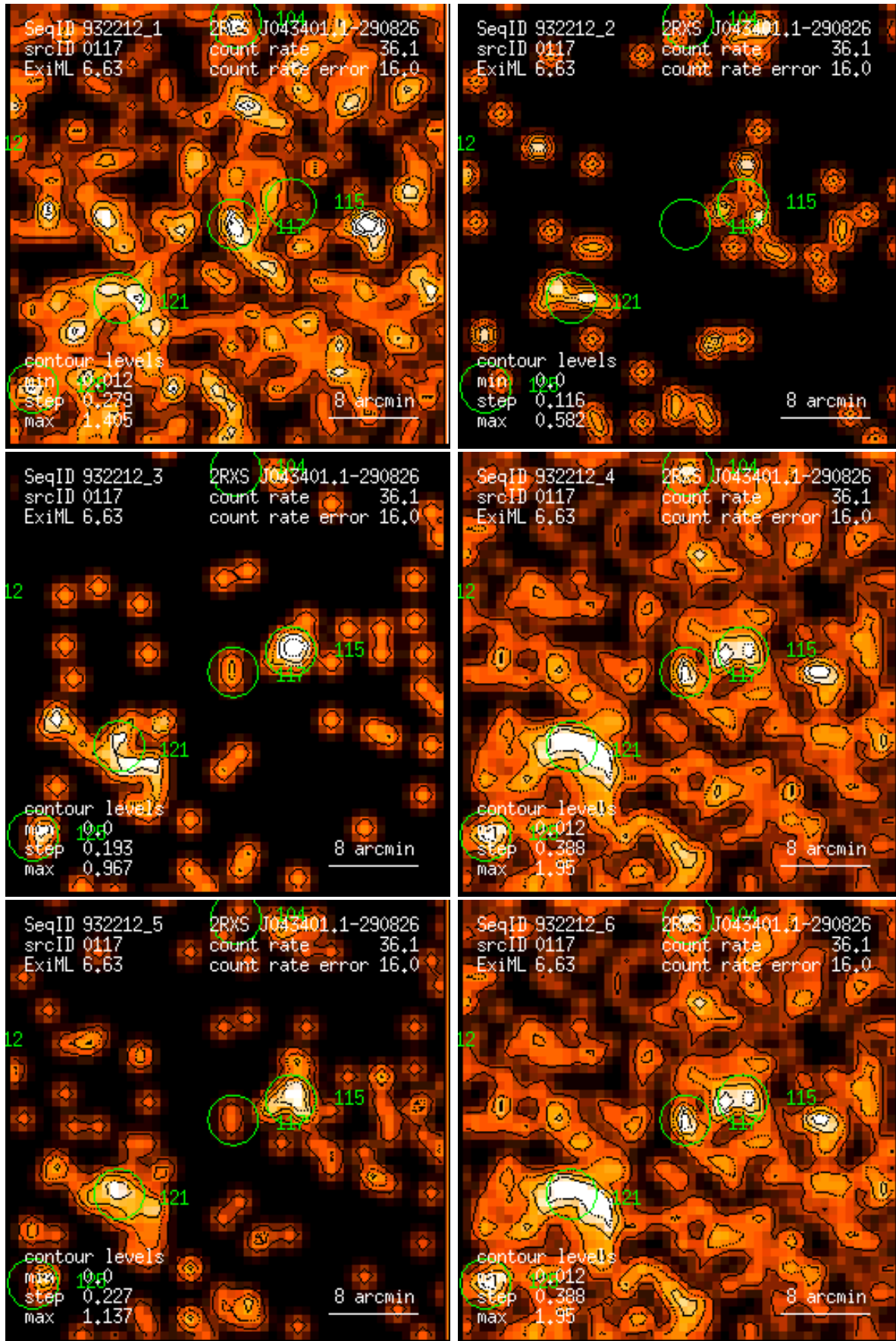
Figure 117: RASS 932212: detection 0117: band rate images, Gaussian filter: (1) PSPC channels 11 – 41, (2) 52 – 90, (3) 91 – 201, (4) 11 – 235, (5) 52 – 201, (6) 11 – 201. Broad band rates in counts/ks. Band rate contour levels in counts/ks/arcmin 2 .
