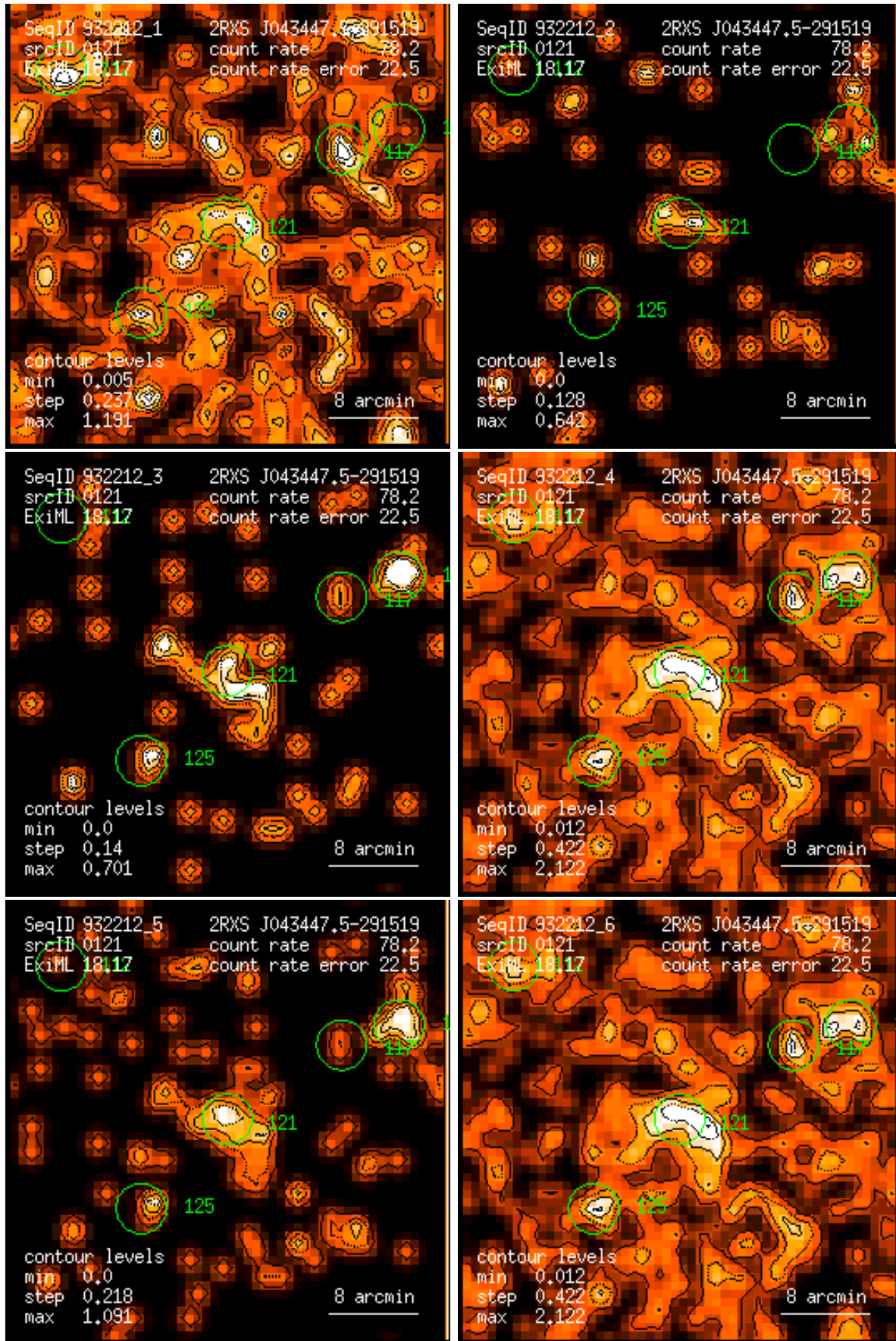
Figure 121: RASS 932212: detection 0121: band rate images, Gaussian filter: (1) PSPC channels 11 – 41, (2) 52 – 90, (3) 91 – 201, (4) 11 – 235, (5) 52 – 201, (6) 11 – 201. Broad band rates in counts/ks. Band rate contour levels in counts/ks/arcmin 2 .
