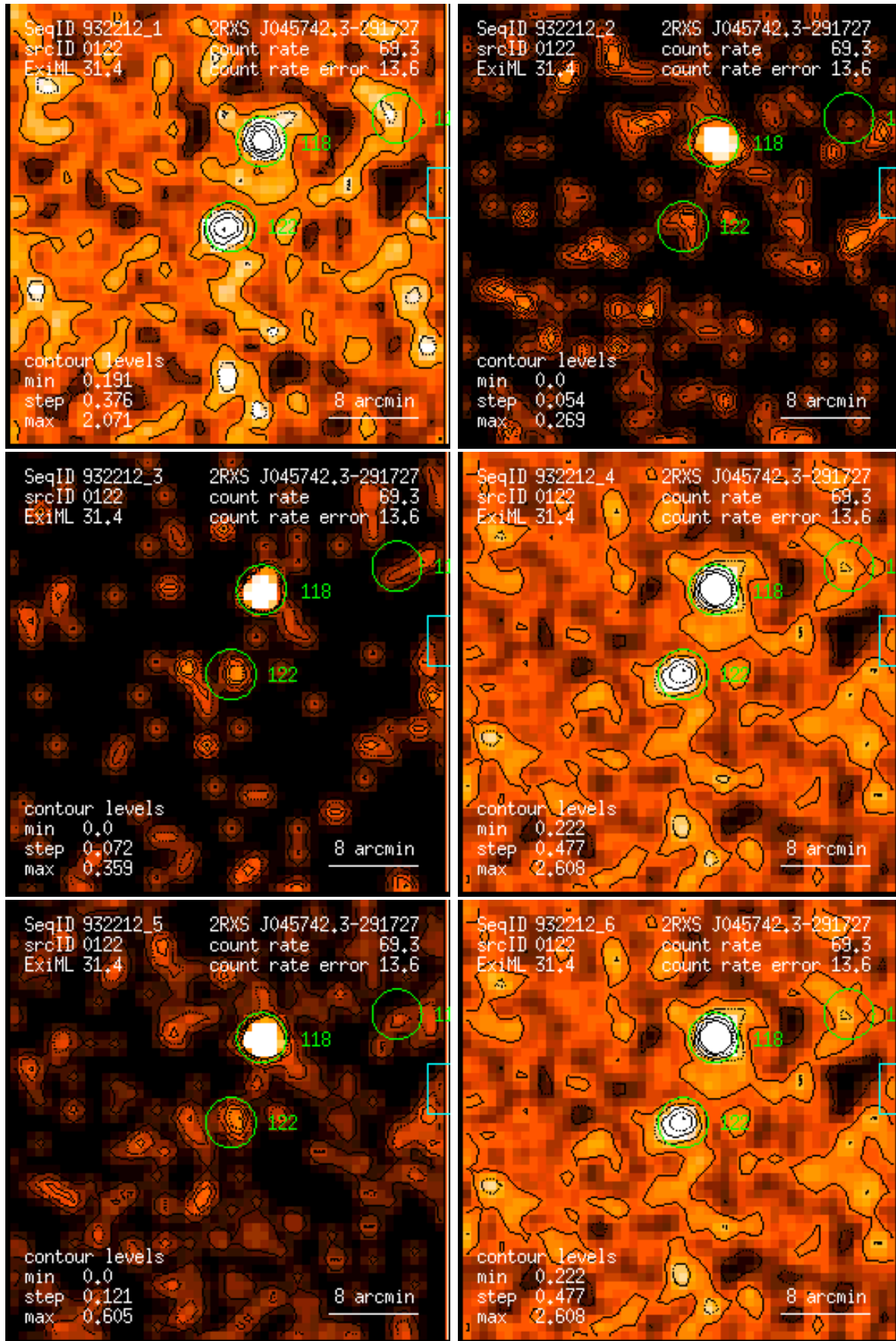
Figure 122: RASS 932212: detection 0122: band rate images, Gaussian filter: (1) PSPC channels 11 – 41, (2) 52 – 90, (3) 91 – 201, (4) 11 – 235, (5) 52 – 201, (6) 11 – 201. Broad band rates in counts/ks. Band rate contour levels in counts/ks/arcmin 2 .
