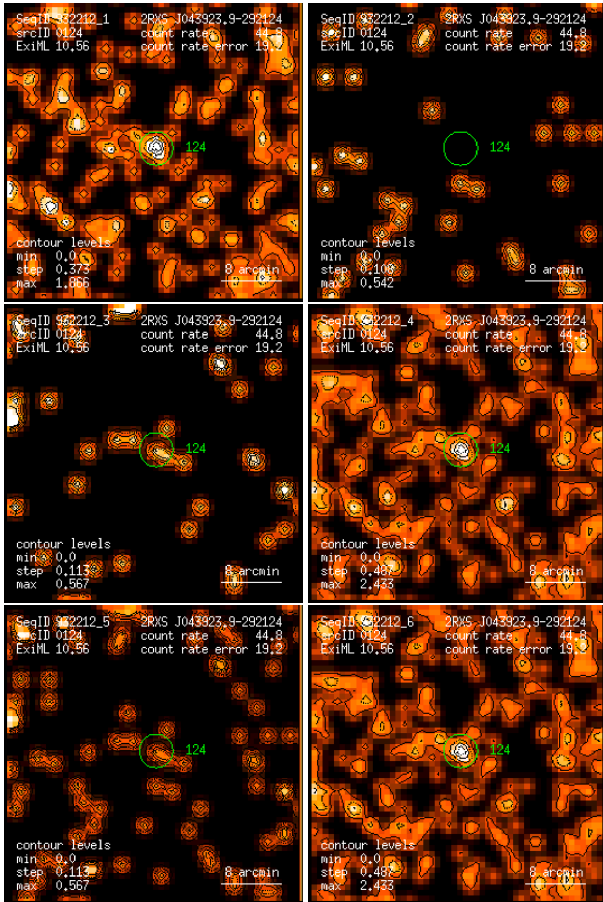
Figure 124: RASS 932212: detection 0124: band rate images, Gaussian filter: (1) PSPC channels 11 – 41, (2) 52 – 90, (3) 91 – 201, (4) 11 – 235, (5) 52 – 201, (6) 11 – 201. Broad band rates in counts/ks. Band rate contour levels in counts/ks/arcmin 2 .
