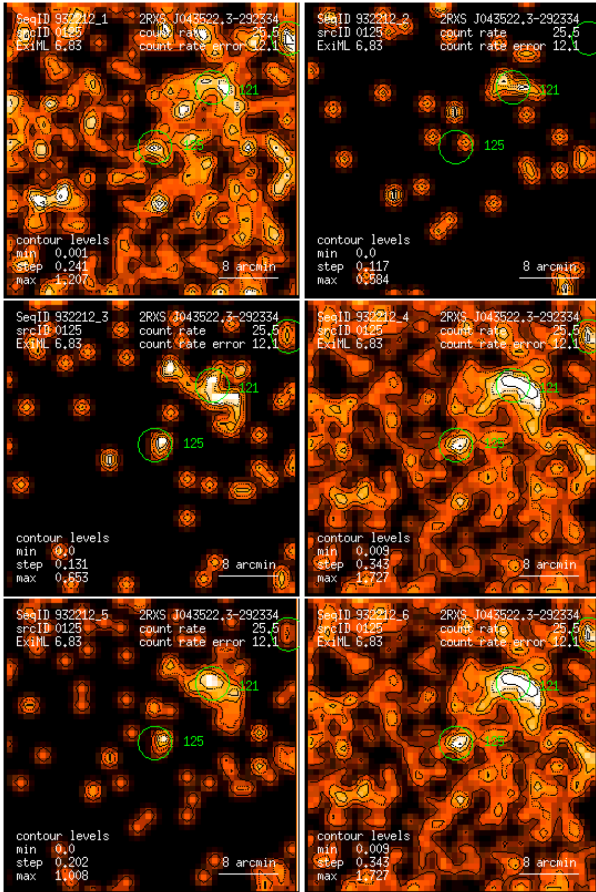
Figure 125: RASS 932212: detection 0125: band rate images, Gaussian filter: (1) PSPC channels 11 – 41, (2) 52 – 90, (3) 91 – 201, (4) 11 – 235, (5) 52 – 201, (6) 11 – 201. Broad band rates in counts/ks. Band rate contour levels in counts/ks/arcmin 2 .
