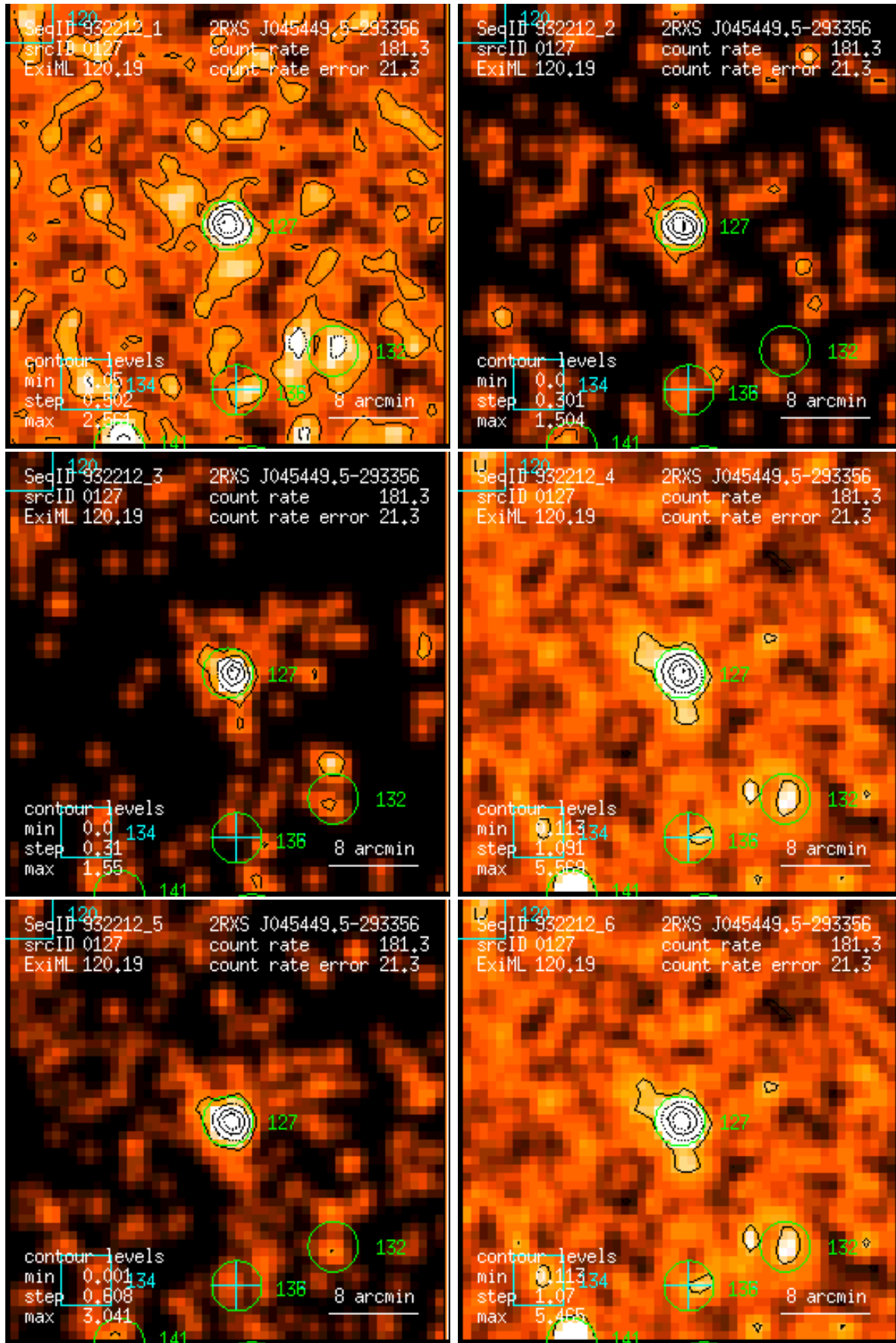
Figure 127: RASS 932212: detection 0127: band rate images, Gaussian filter: (1) PSPC channels 11 – 41, (2) 52 – 90, (3) 91 – 201, (4) 11 – 235, (5) 52 – 201, (6) 11 – 201. Broad band rates in counts/ks. Band rate contour levels in counts/ks/arcmin 2 .
