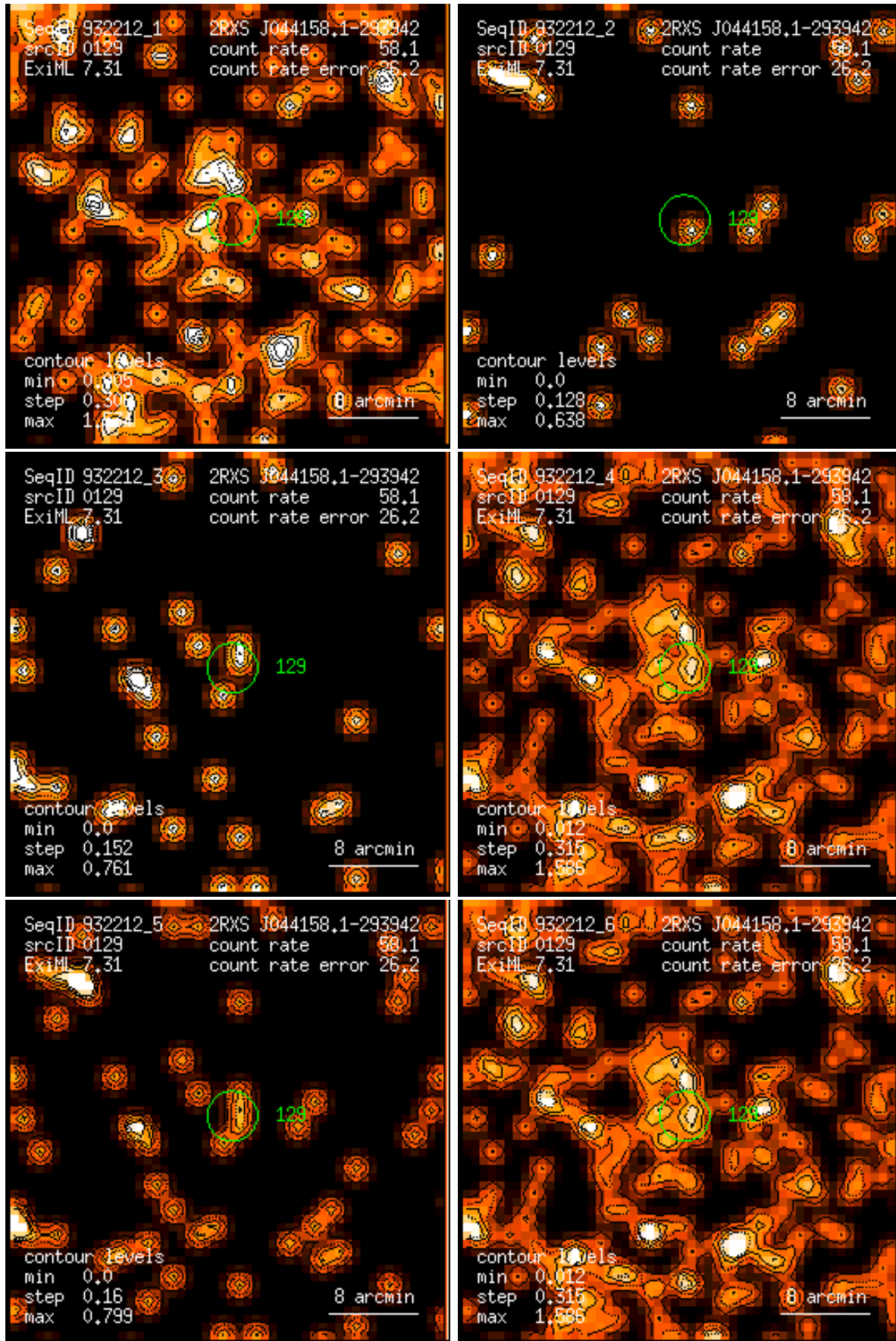
Figure 129: RASS 932212: detection 0129: band rate images, Gaussian filter: (1) PSPC channels 11 – 41, (2) 52 – 90, (3) 91 – 201, (4) 11 – 235, (5) 52 – 201, (6) 11 – 201. Broad band rates in counts/ks. Band rate contour levels in counts/ks/arcmin 2 .
