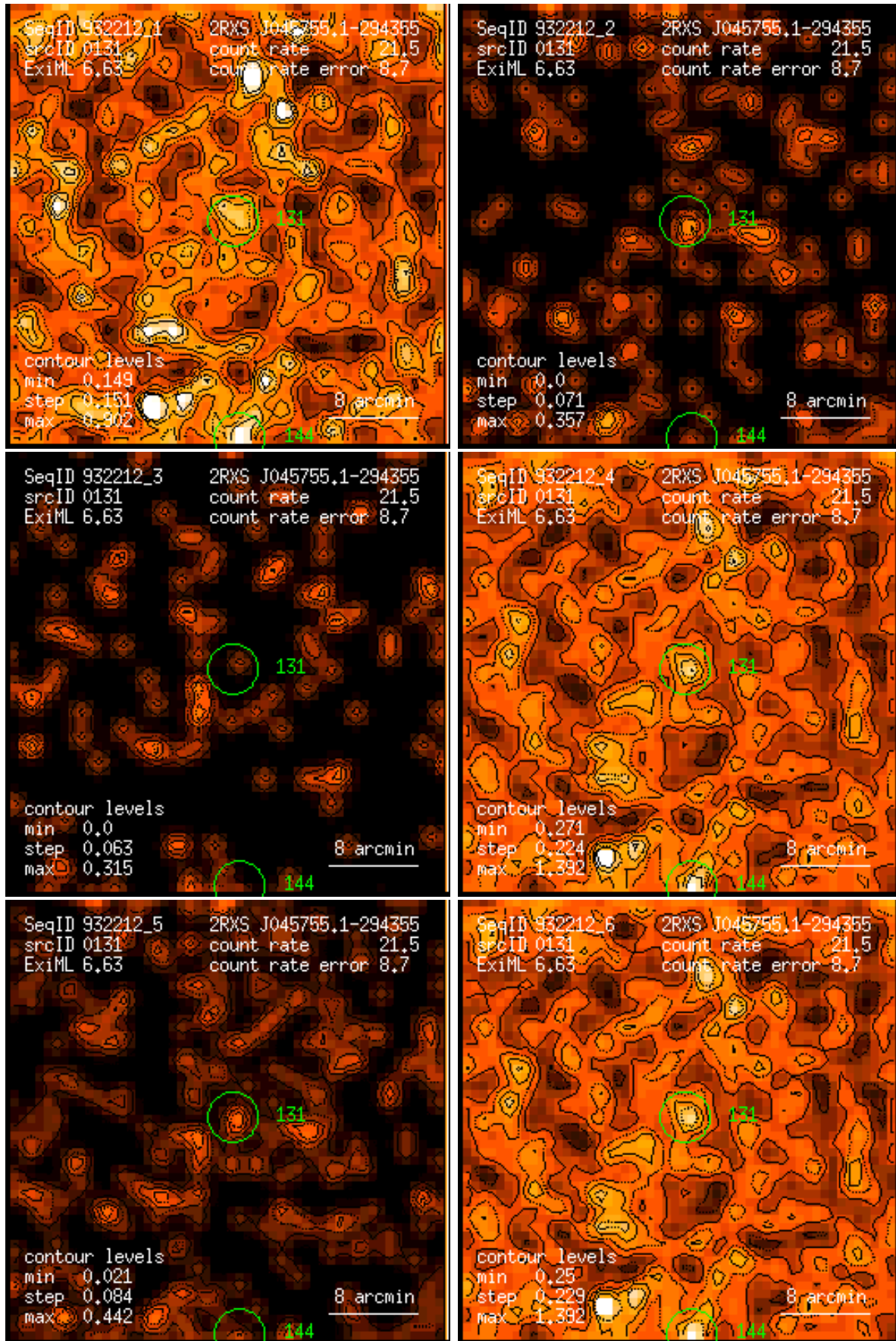
Figure 131: RASS 932212: detection 0131: band rate images, Gaussian filter: (1) PSPC channels 11 – 41, (2) 52 – 90, (3) 91 – 201, (4) 11 – 235, (5) 52 – 201, (6) 11 – 201. Broad band rates in counts/ks. Band rate contour levels in counts/ks/arcmin 2 .
