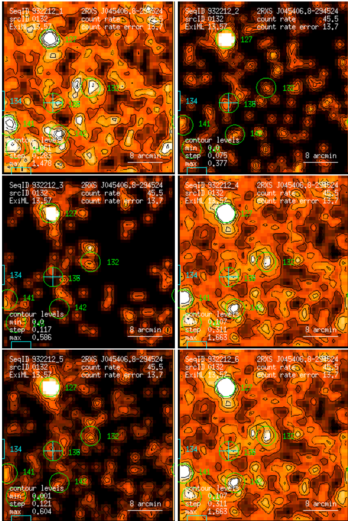
Figure 132: RASS 932212: detection 0132: band rate images, Gaussian filter: (1) PSPC channels 11 – 41, (2) 52 – 90, (3) 91 – 201, (4) 11 – 235, (5) 52 – 201, (6) 11 – 201. Broad band rates in counts/ks. Band rate contour levels in counts/ks/arcmin 2 .
