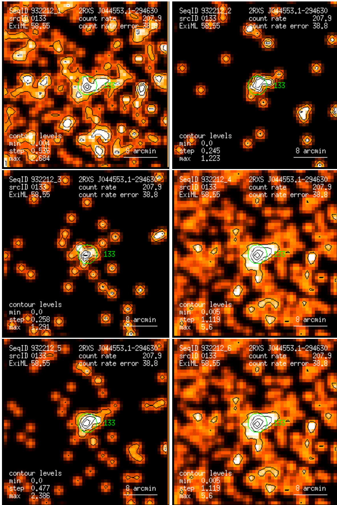
Figure 133: RASS 932212: detection 0133: band rate images, Gaussian filter: (1) PSPC channels 11 – 41, (2) 52 – 90, (3) 91 – 201, (4) 11 – 235, (5) 52 – 201, (6) 11 – 201. Broad band rates in counts/ks. Band rate contour levels in counts/ks/arcmin 2 .
