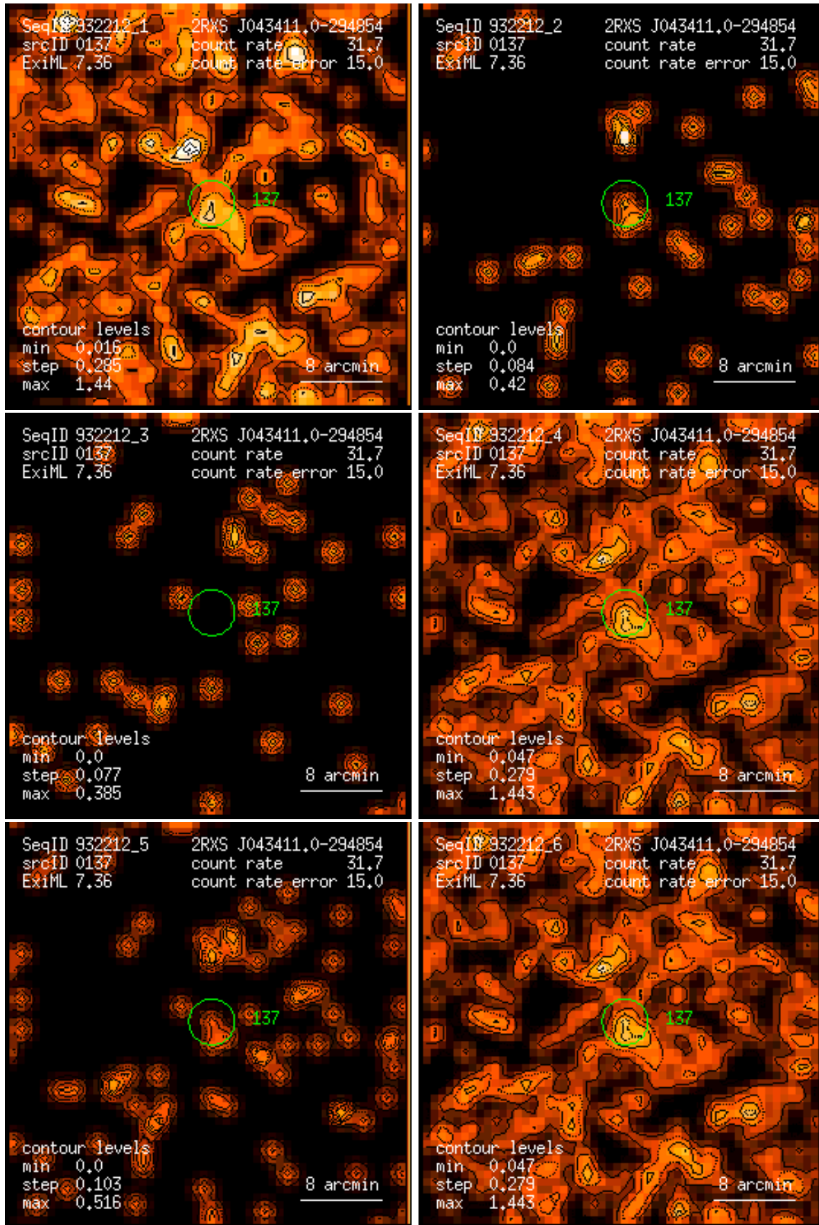
Figure 137: RASS 932212: detection 0137: band rate images, Gaussian filter: (1) PSPC channels 11 – 41, (2) 52 – 90, (3) 91 – 201, (4) 11 – 235, (5) 52 – 201, (6) 11 – 201. Broad band rates in counts/ks. Band rate contour levels in counts/ks/arcmin 2 .
