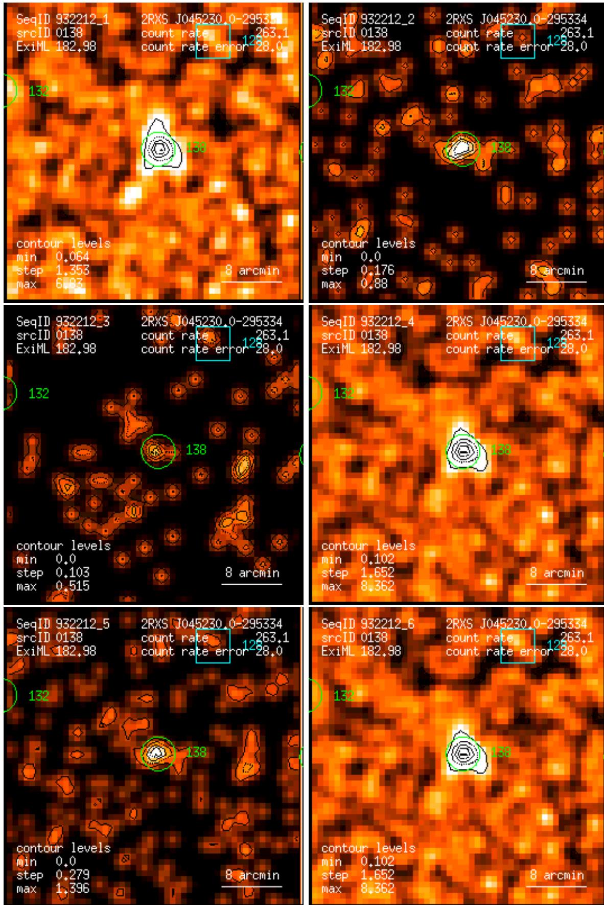
Figure 138: RASS 932212: detection 0138: band rate images, Gaussian filter: (1) PSPC channels 11 – 41, (2) 52 – 90, (3) 91 – 201, (4) 11 – 235, (5) 52 – 201, (6) 11 – 201. Broad band rates in counts/ks. Band rate contour levels in counts/ks/arcmin 2 .
