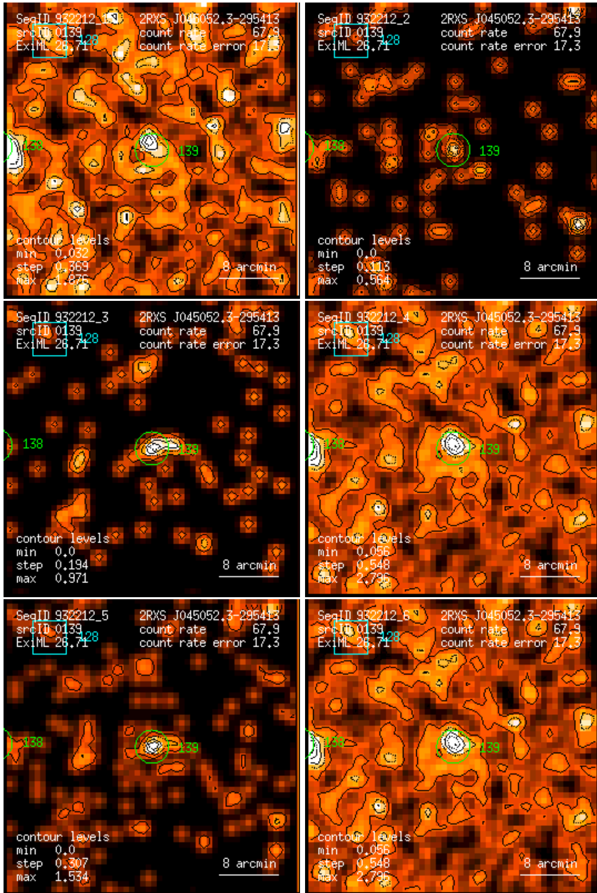
Figure 139: RASS 932212: detection 0139: band rate images, Gaussian filter: (1) PSPC channels 11 – 41, (2) 52 – 90, (3) 91 – 201, (4) 11 – 235, (5) 52 – 201, (6) 11 – 201. Broad band rates in counts/ks. Band rate contour levels in counts/ks/arcmin 2 .
