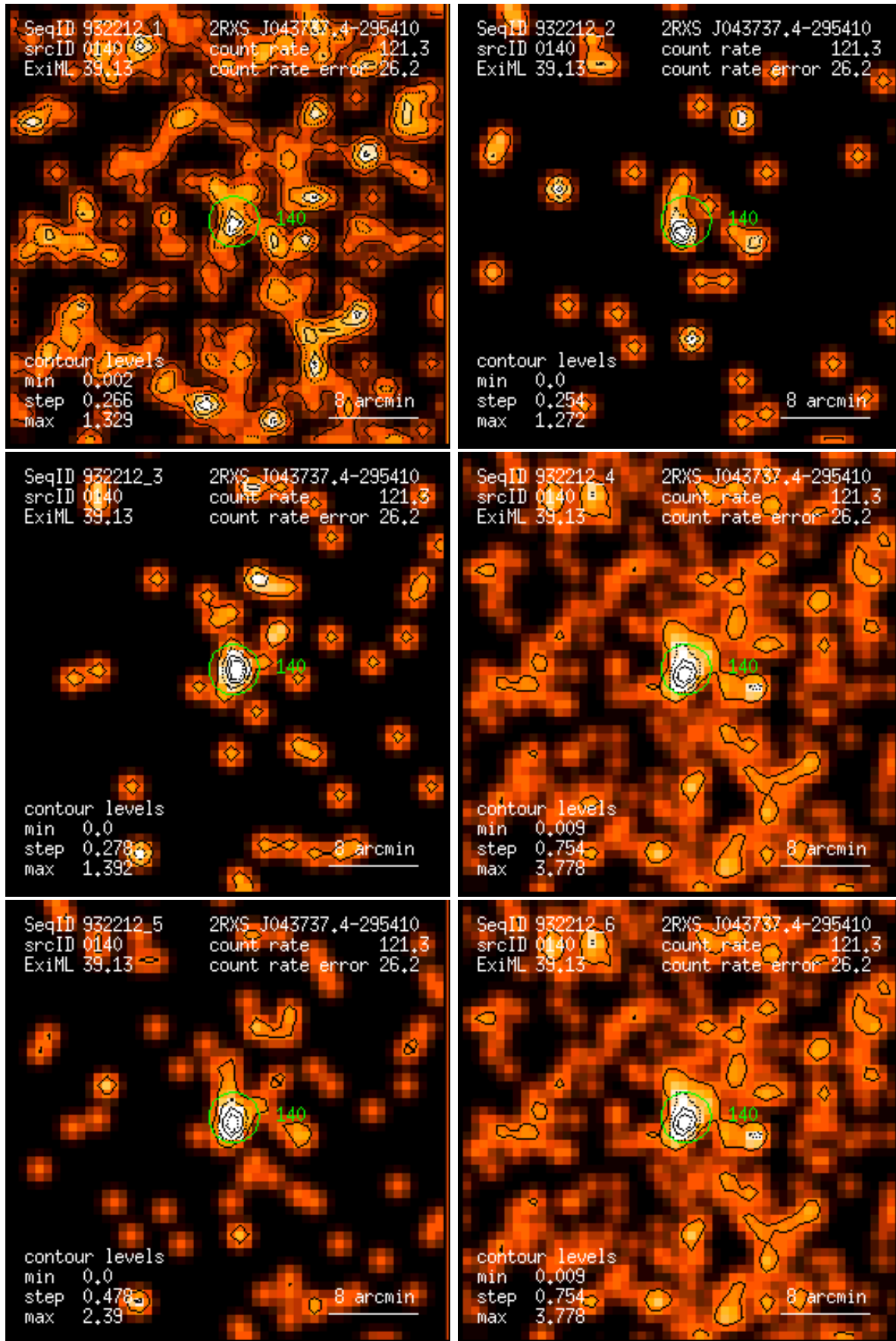
Figure 140: RASS 932212: detection 0140: band rate images, Gaussian filter: (1) PSPC channels 11 – 41, (2) 52 – 90, (3) 91 – 201, (4) 11 – 235, (5) 52 – 201, (6) 11 – 201. Broad band rates in counts/ks. Band rate contour levels in counts/ks/arcmin 2 .
