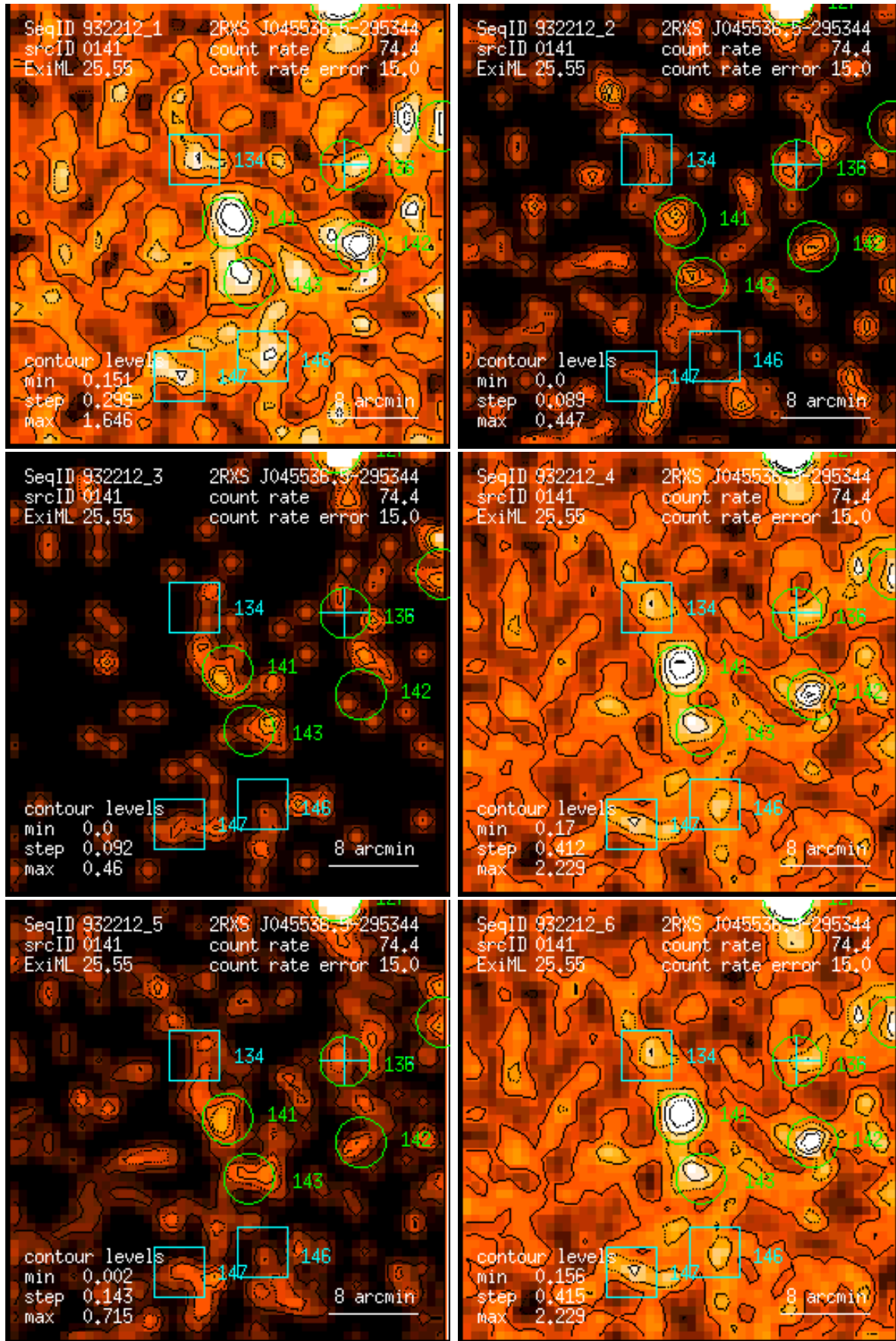
Figure 141: RASS 932212: detection 0141: band rate images, Gaussian filter: (1) PSPC channels 11 – 41, (2) 52 – 90, (3) 91 – 201, (4) 11 – 235, (5) 52 – 201, (6) 11 – 201. Broad band rates in counts/ks. Band rate contour levels in counts/ks/arcmin 2 .
