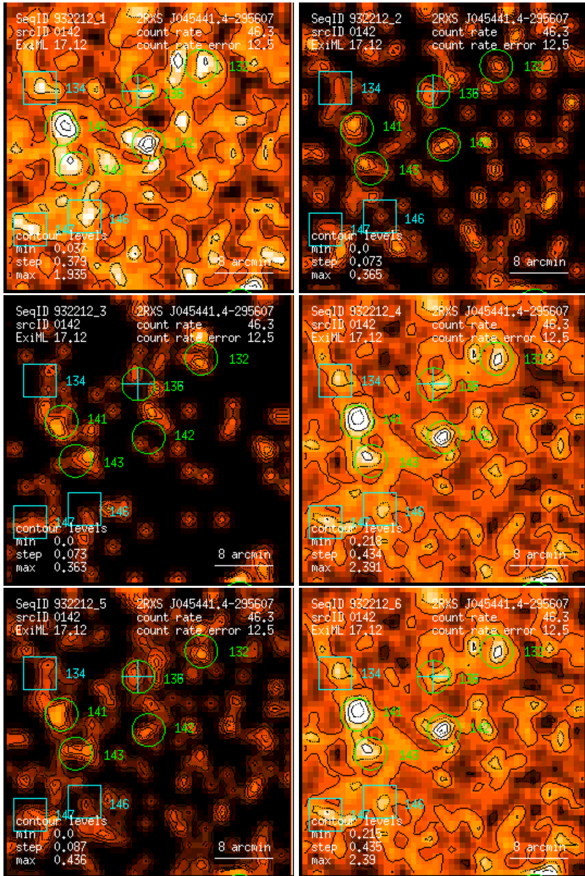
Figure 142: RASS 932212: detection 0142: band rate images, Gaussian filter: (1) PSPC channels 11 – 41, (2) 52 – 90, (3) 91 – 201, (4) 11 – 235, (5) 52 – 201, (6) 11 – 201. Broad band rates in counts/ks. Band rate contour levels in counts/ks/arcmin 2 .
