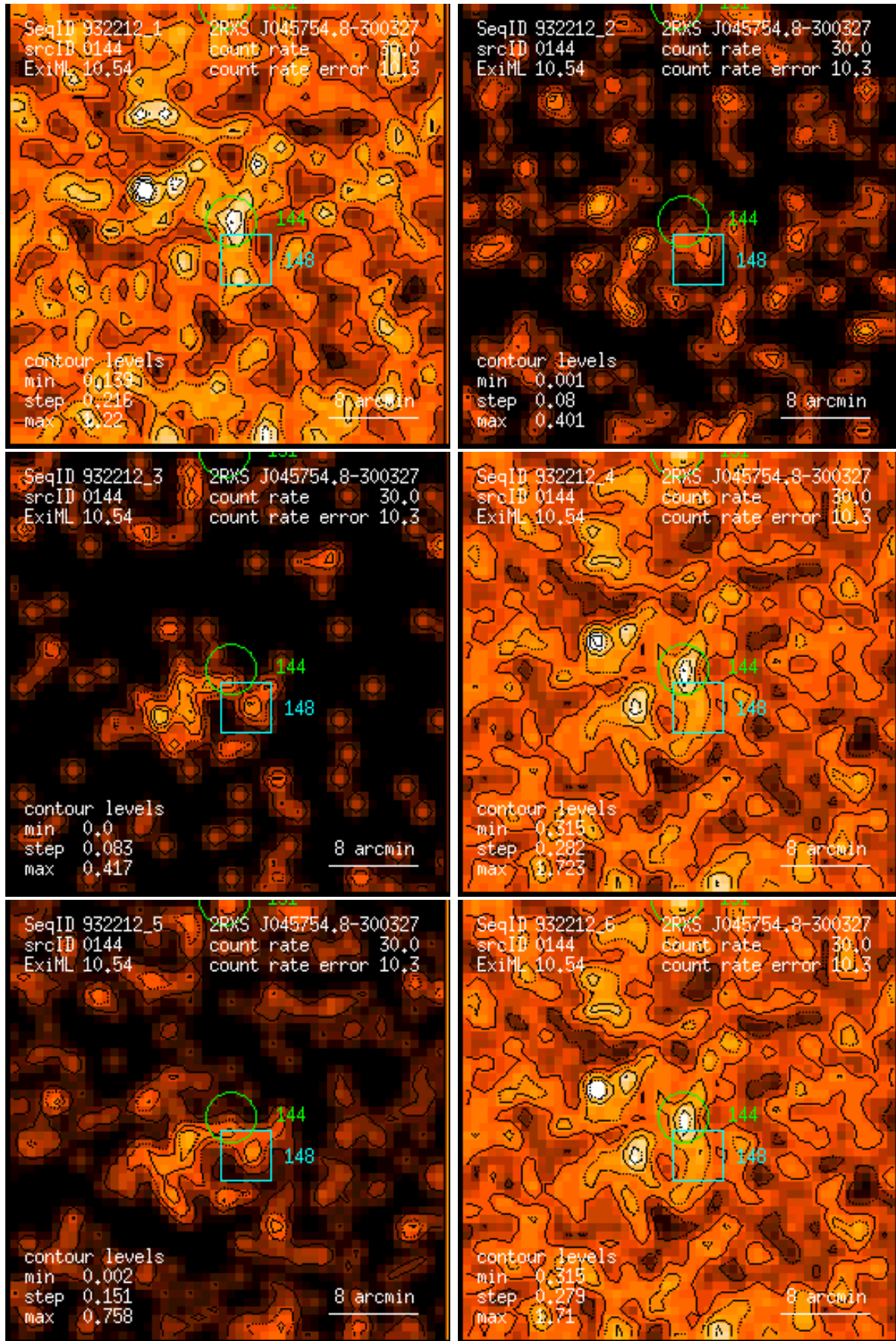
Figure 144: RASS 932212: detection 0144: band rate images, Gaussian filter: (1) PSPC channels 11 – 41, (2) 52 – 90, (3) 91 – 201, (4) 11 – 235, (5) 52 – 201, (6) 11 – 201. Broad band rates in counts/ks. Band rate contour levels in counts/ks/arcmin 2 .
